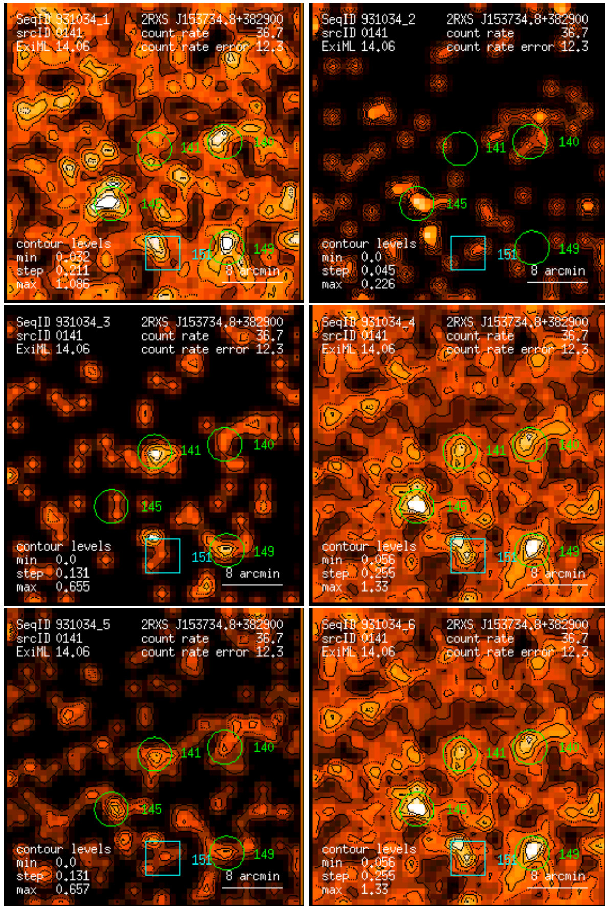
Figure 141: RASS 931034: detection 0141: band rate images, Gaussian filter: (1) PSPC channels 11 – 41, (2) 52 – 90, (3) 91 – 201, (4) 11 – 235, (5) 52 – 201, (6) 11 – 201. Broad band rates in counts/ks. Band rate contour levels in counts/ks/arcmin 2 .
