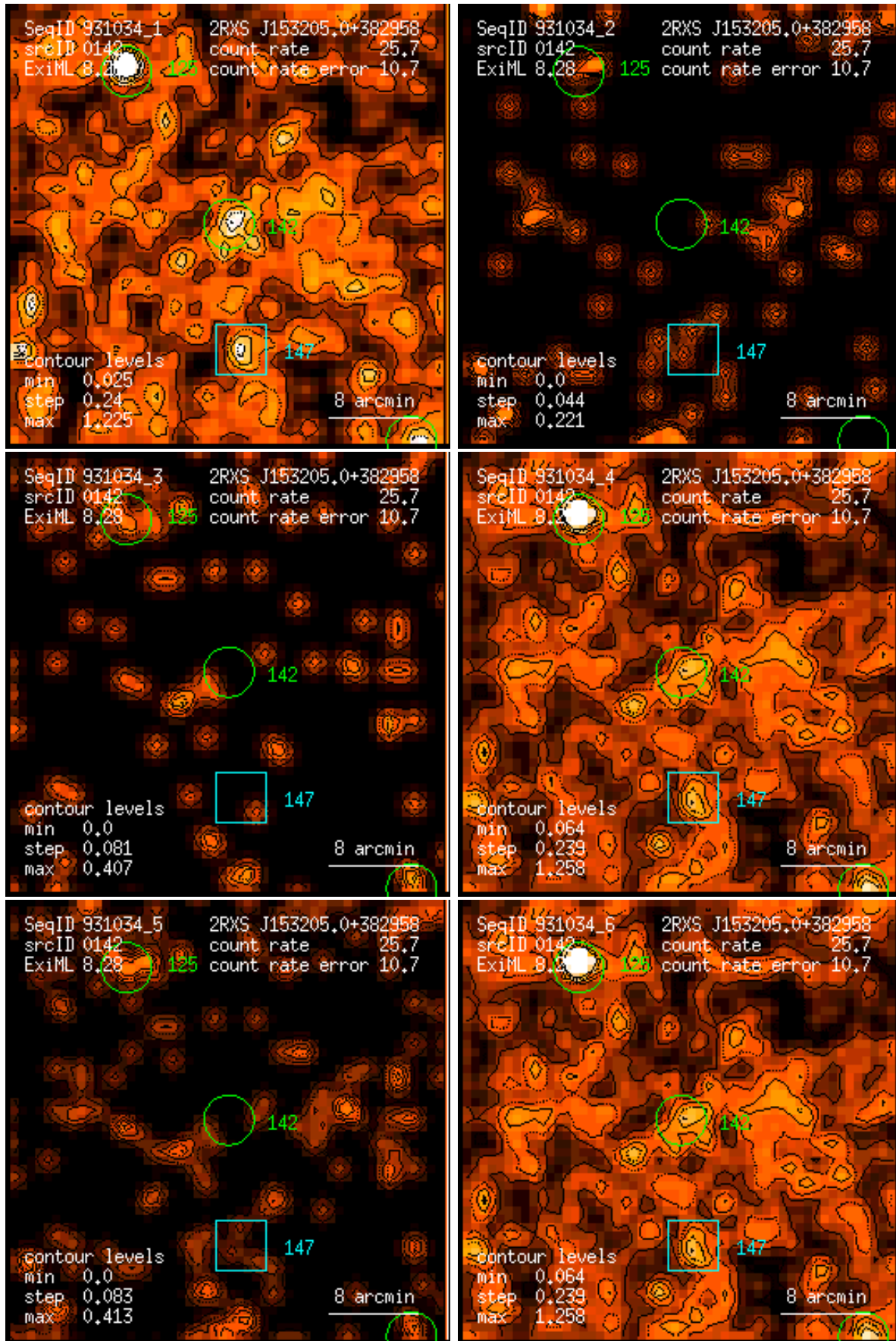
Figure 142: RASS 931034: detection 0142: band rate images, Gaussian filter: (1) PSPC channels 11 – 41, (2) 52 – 90, (3) 91 – 201, (4) 11 – 235, (5) 52 – 201, (6) 11 – 201. Broad band rates in counts/ks. Band rate contour levels in counts/ks/arcmin 2 .
