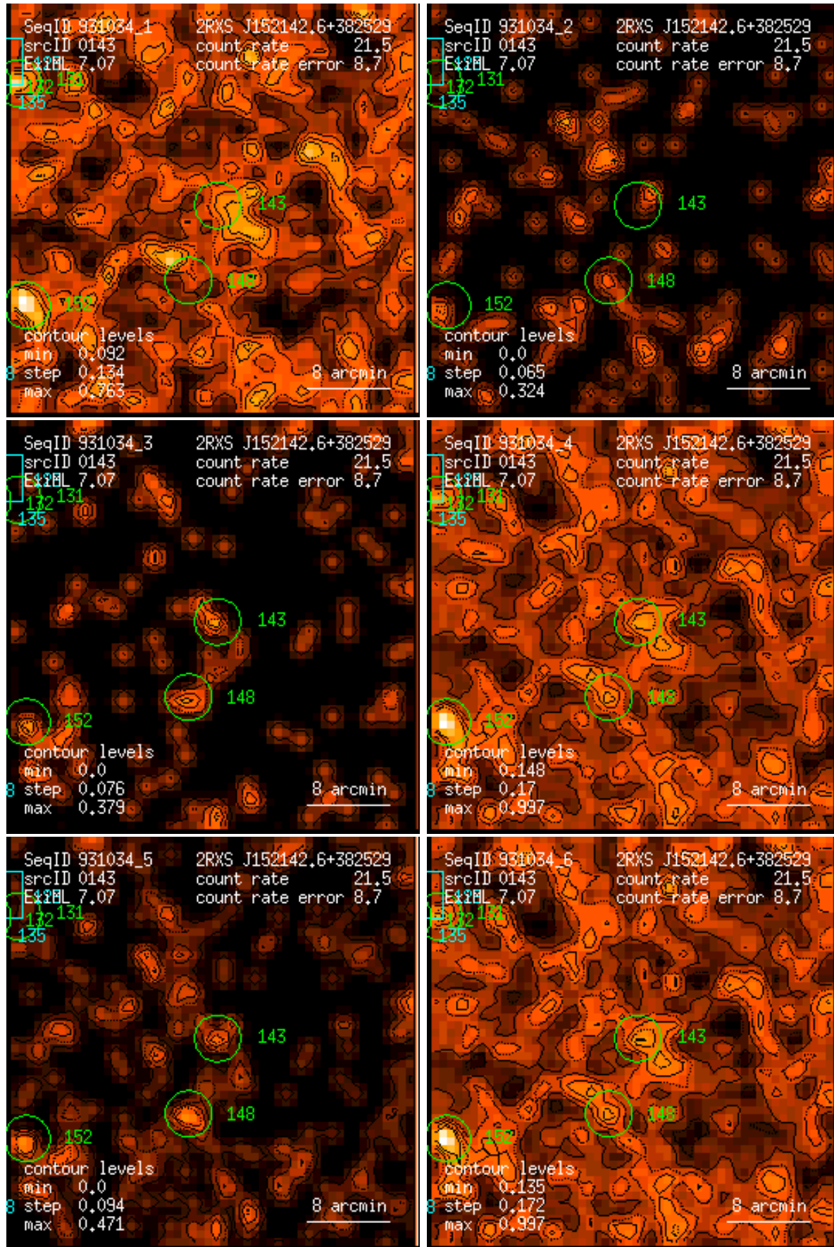
Figure 143: RASS 931034: detection 0143: band rate images, Gaussian filter: (1) PSPC channels 11 – 41, (2) 52 – 90, (3) 91 – 201, (4) 11 – 235, (5) 52 – 201, (6) 11 – 201. Broad band rates in counts/ks. Band rate contour levels in counts/ks/arcmin 2 .
