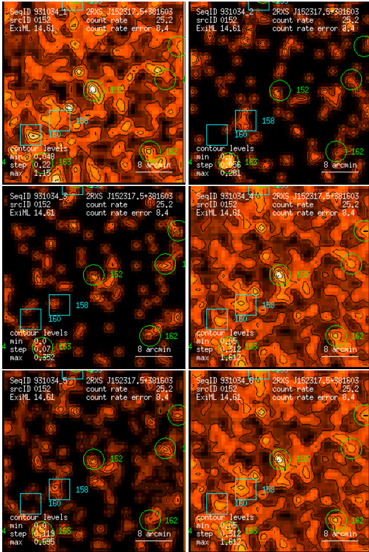
Figure 152: RASS 931034: detection 0152: band rate images, Gaussian filter: (1) PSPC channels 11 – 41, (2) 52 – 90, (3) 91 – 201, (4) 11 – 235, (5) 52 – 201, (6) 11 – 201. Broad band rates in counts/ks. Band rate contour levels in counts/ks/arcmin 2 .
