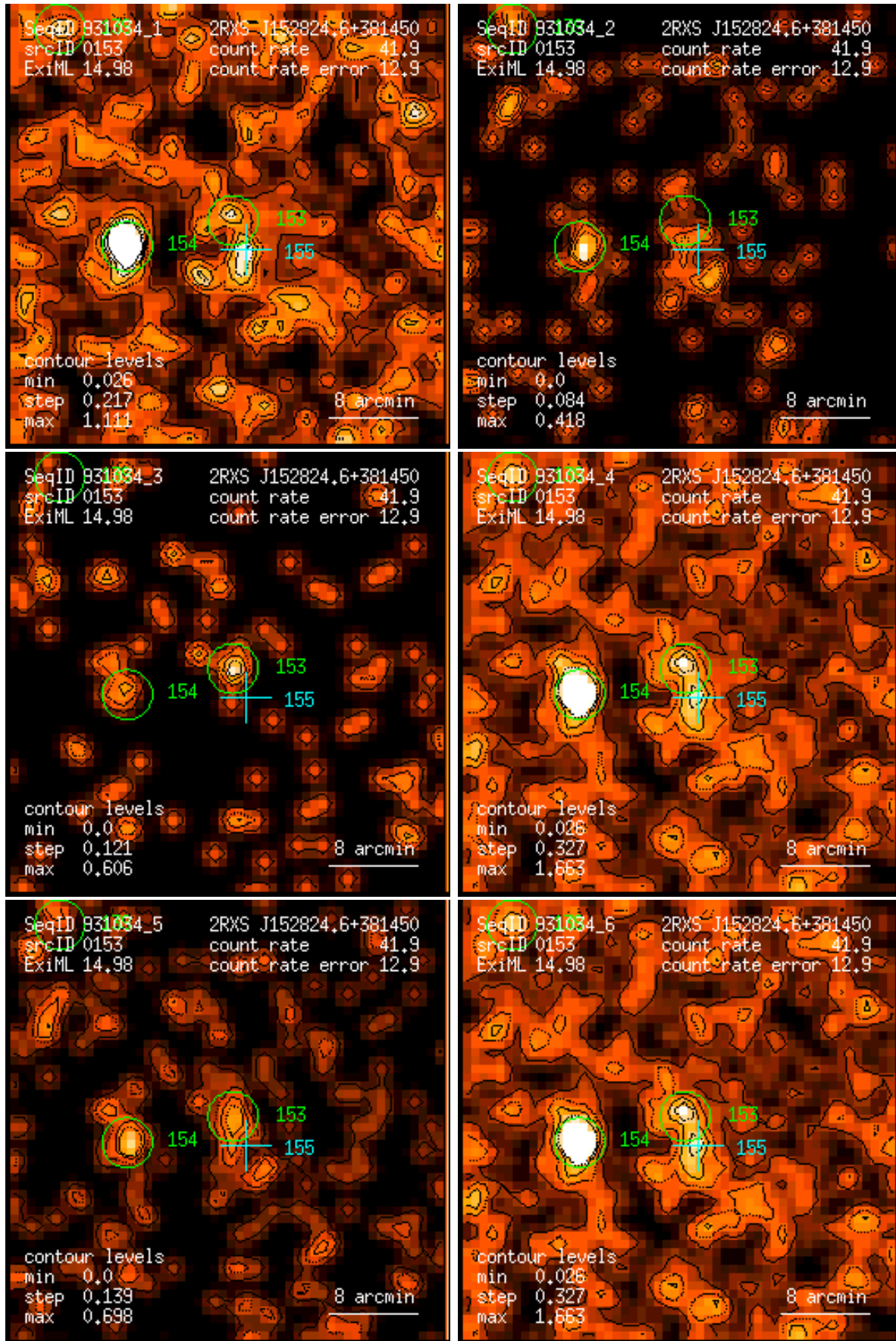
Figure 153: RASS 931034: detection 0153: band rate images, Gaussian filter: (1) PSPC channels 11 – 41, (2) 52 – 90, (3) 91 – 201, (4) 11 – 235, (5) 52 – 201, (6) 11 – 201. Broad band rates in counts/ks. Band rate contour levels in counts/ks/arcmin 2 .
