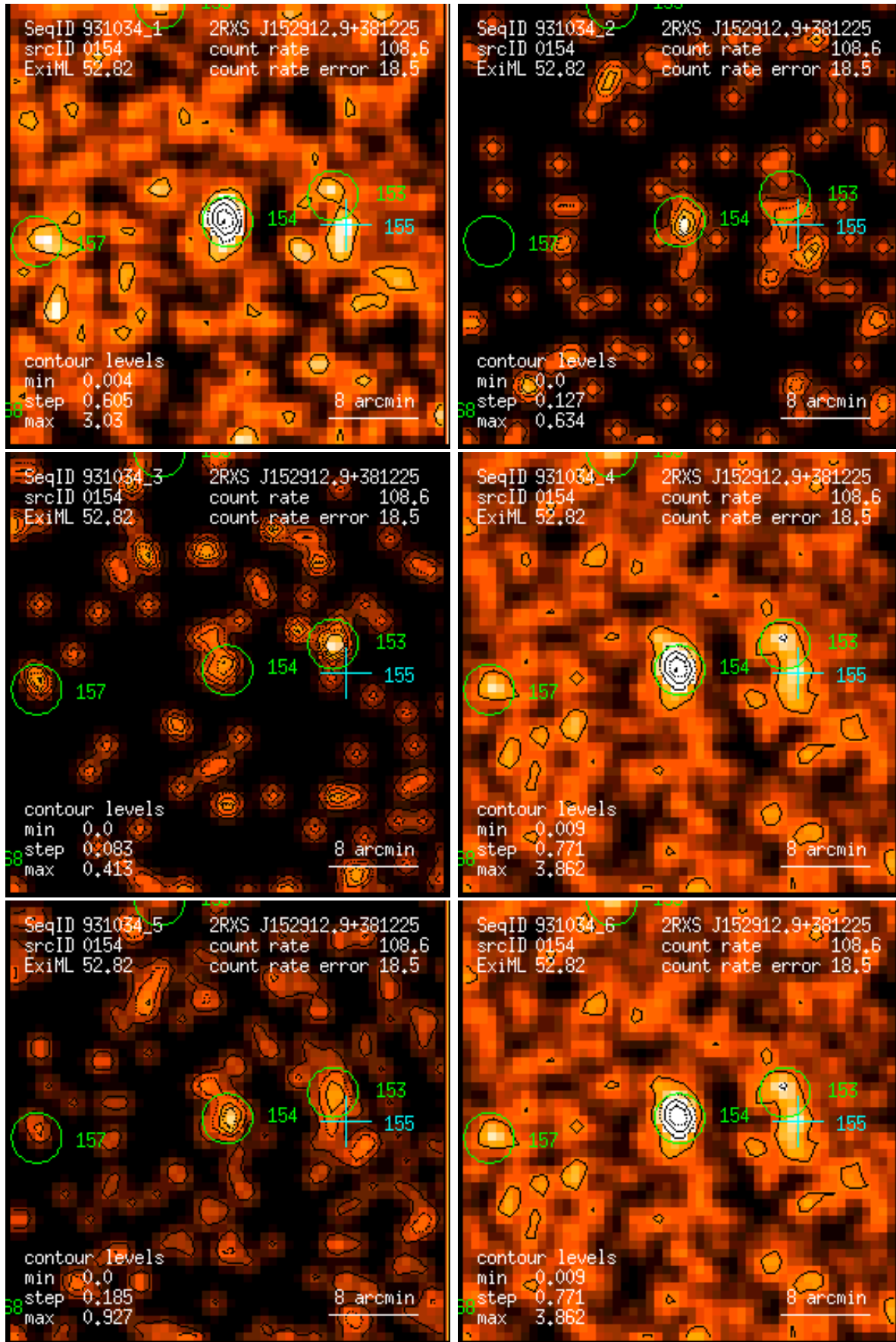
Figure 154: RASS 931034: detection 0154: band rate images, Gaussian filter: (1) PSPC channels 11 – 41, (2) 52 – 90, (3) 91 – 201, (4) 11 – 235, (5) 52 – 201, (6) 11 – 201. Broad band rates in counts/ks. Band rate contour levels in counts/ks/arcmin 2 .
