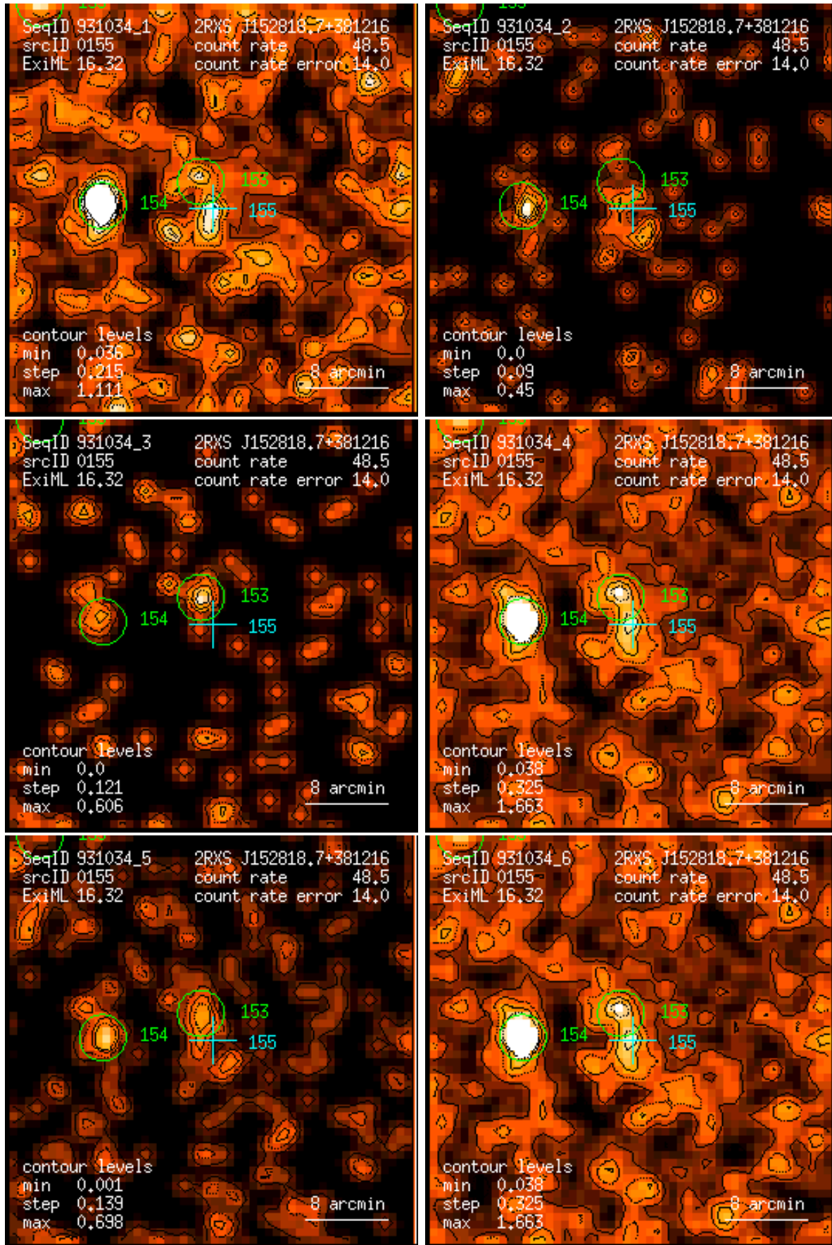
Figure 155: RASS 931034: detection 0155: band rate images, Gaussian filter: (1) PSPC channels 11 – 41, (2) 52 – 90, (3) 91 – 201, (4) 11 – 235, (5) 52 – 201, (6) 11 – 201. Broad band rates in counts/ks. Band rate contour levels in counts/ks/arcmin 2 .
