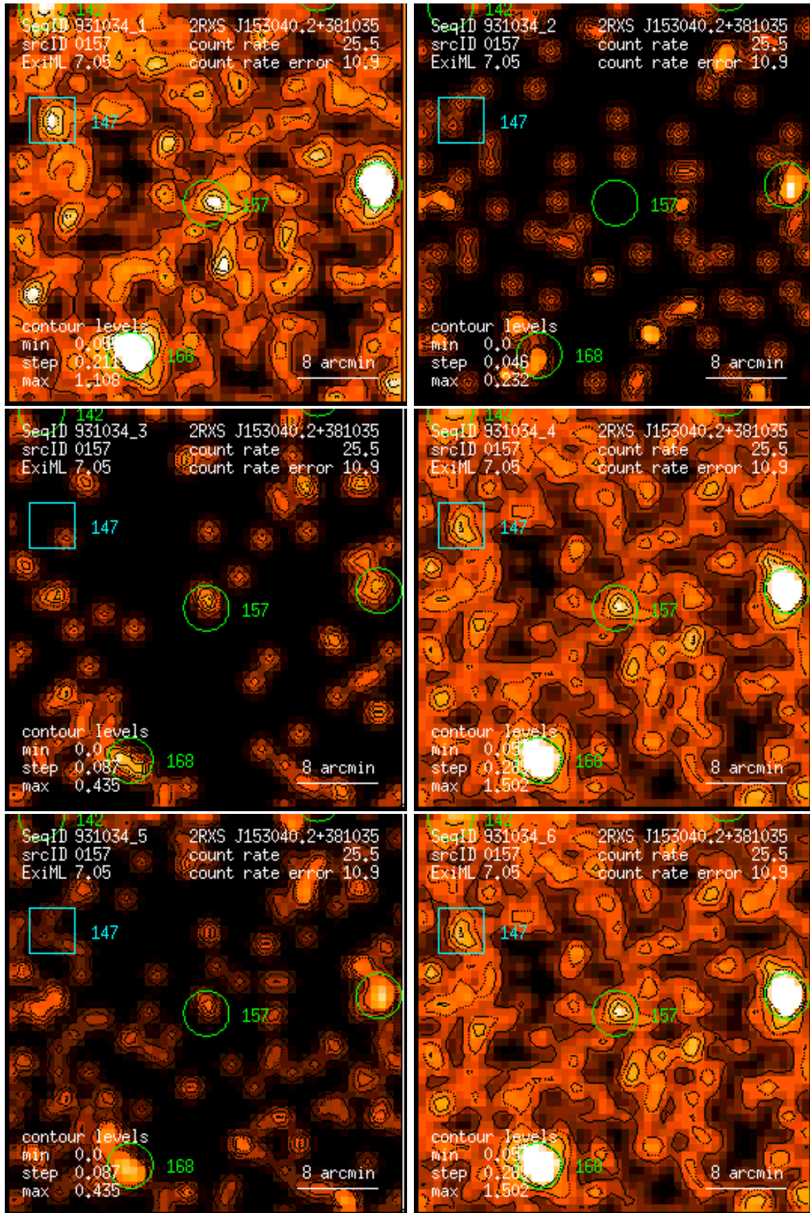
Figure 157: RASS 931034: detection 0157: band rate images, Gaussian filter: (1) PSPC channels 11 – 41, (2) 52 – 90, (3) 91 – 201, (4) 11 – 235, (5) 52 – 201, (6) 11 – 201. Broad band rates in counts/ks. Band rate contour levels in counts/ks/arcmin 2 .
