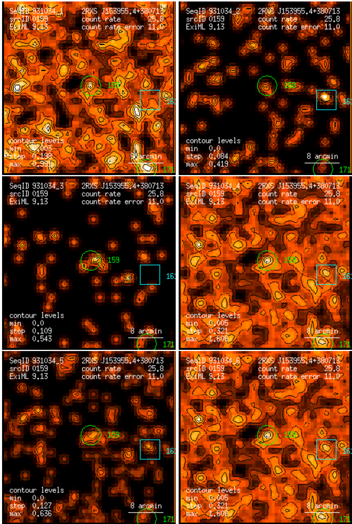
Figure 159: RASS 931034: detection 0159: band rate images, Gaussian filter: (1) PSPC channels 11 – 41, (2) 52 – 90, (3) 91 – 201, (4) 11 – 235, (5) 52 – 201, (6) 11 – 201. Broad band rates in counts/ks. Band rate contour levels in counts/ks/arcmin 2 .
