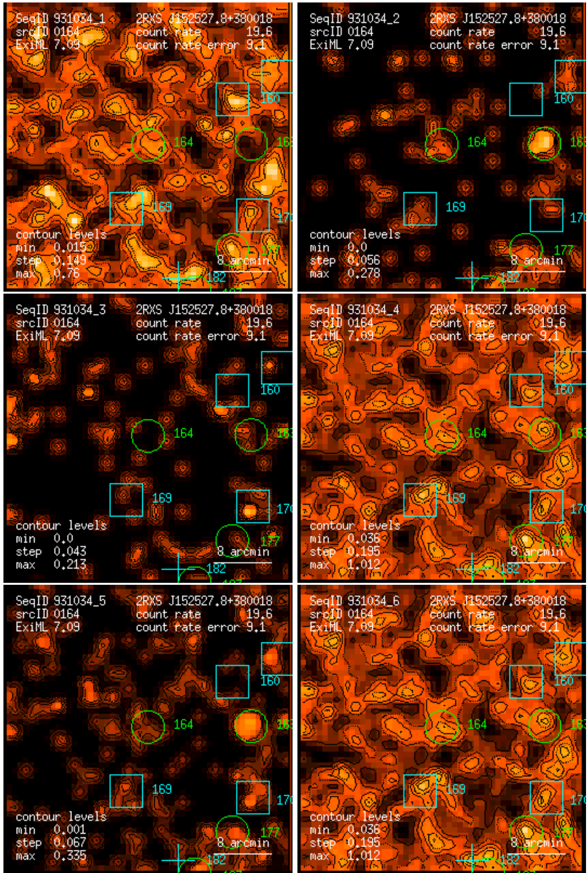
Figure 164: RASS 931034: detection 0164: band rate images, Gaussian filter: (1) PSPC channels 11 – 41, (2) 52 – 90, (3) 91 – 201, (4) 11 – 235, (5) 52 – 201, (6) 11 – 201. Broad band rates in counts/ks. Band rate contour levels in counts/ks/arcmin 2 .
