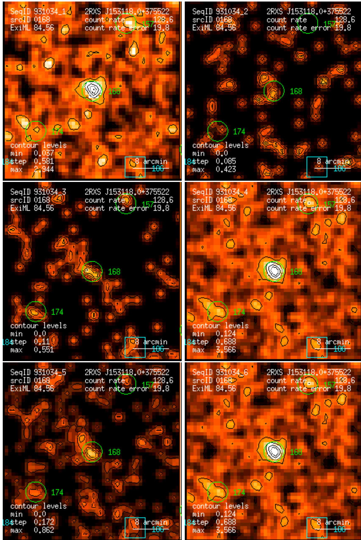
Figure 168: RASS 931034: detection 0168: band rate images, Gaussian filter: (1) PSPC channels 11 – 41, (2) 52 – 90, (3) 91 – 201, (4) 11 – 235, (5) 52 – 201, (6) 11 – 201. Broad band rates in counts/ks. Band rate contour levels in counts/ks/arcmin 2 .
