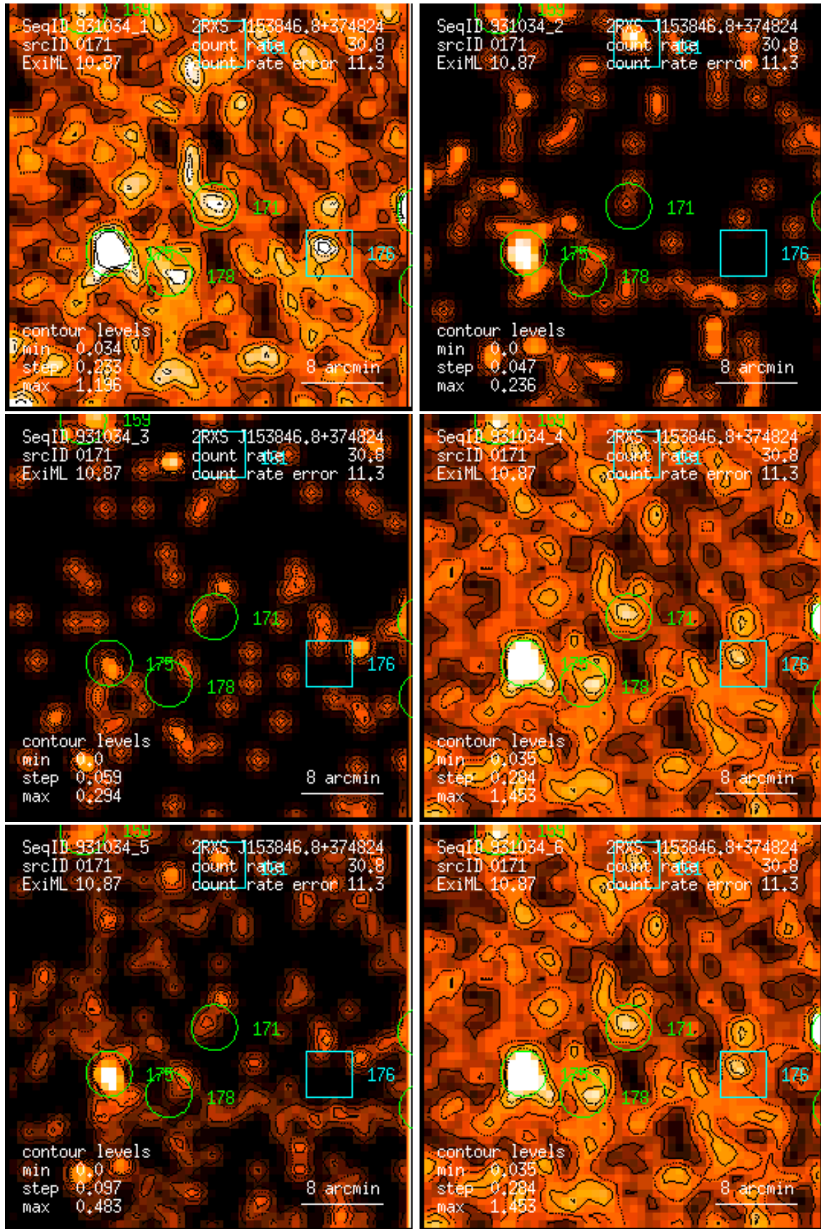
Figure 171: RASS 931034: detection 0171: band rate images, Gaussian filter: (1) PSPC channels 11 – 41, (2) 52 – 90, (3) 91 – 201, (4) 11 – 235, (5) 52 – 201, (6) 11 – 201. Broad band rates in counts/ks. Band rate contour levels in counts/ks/arcmin 2 .
