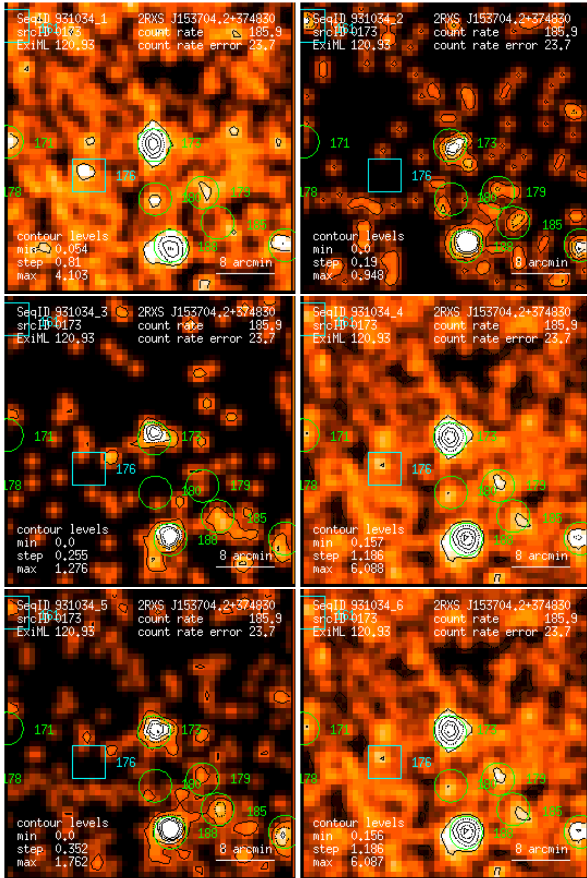
Figure 173: RASS 931034: detection 0173: band rate images, Gaussian filter: (1) PSPC channels 11 – 41, (2) 52 – 90, (3) 91 – 201, (4) 11 – 235, (5) 52 – 201, (6) 11 – 201. Broad band rates in counts/ks. Band rate contour levels in counts/ks/arcmin 2 .
