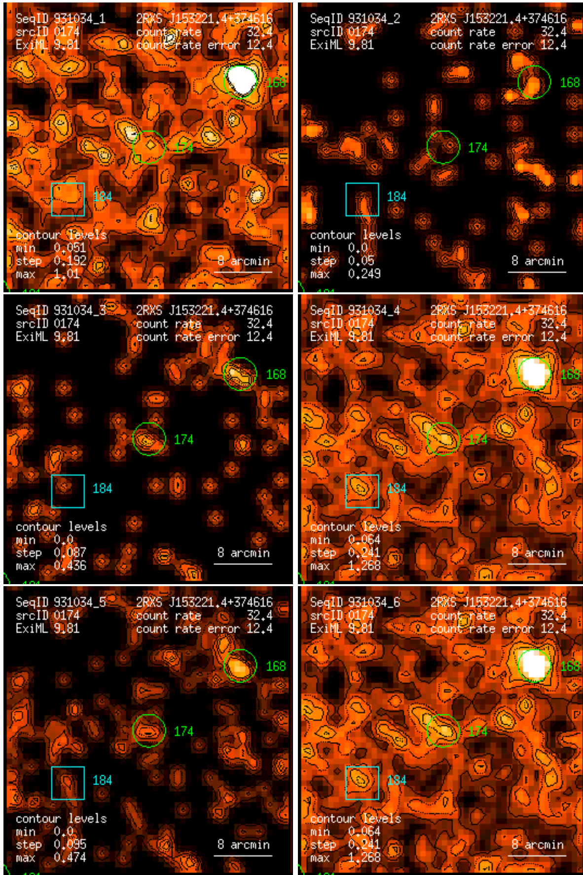
Figure 174: RASS 931034: detection 0174: band rate images, Gaussian filter: (1) PSPC channels 11 – 41, (2) 52 – 90, (3) 91 – 201, (4) 11 – 235, (5) 52 – 201, (6) 11 – 201. Broad band rates in counts/ks. Band rate contour levels in counts/ks/arcmin 2 .
