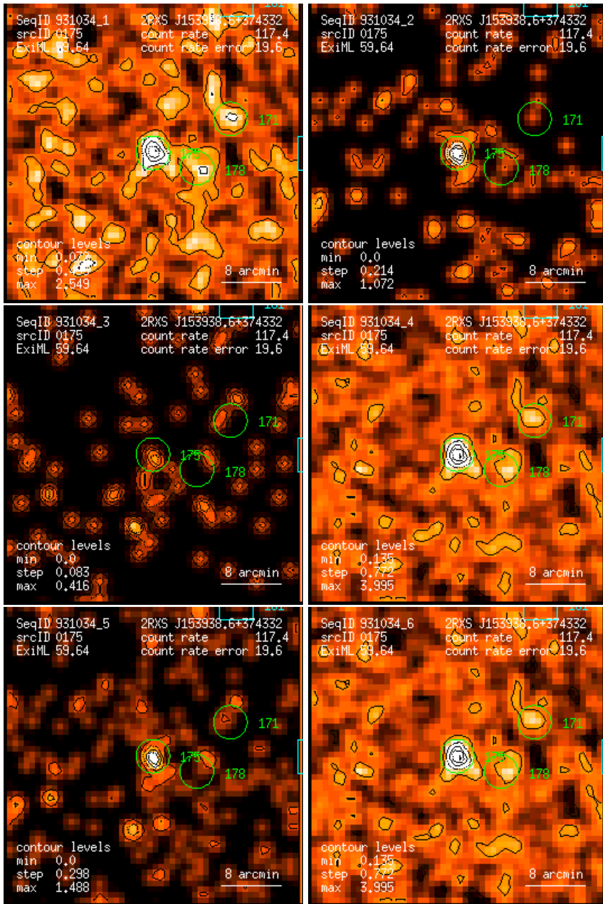
Figure 175: RASS 931034: detection 0175: band rate images, Gaussian filter: (1) PSPC channels 11 – 41, (2) 52 – 90, (3) 91 – 201, (4) 11 – 235, (5) 52 – 201, (6) 11 – 201. Broad band rates in counts/ks. Band rate contour levels in counts/ks/arcmin 2 .
