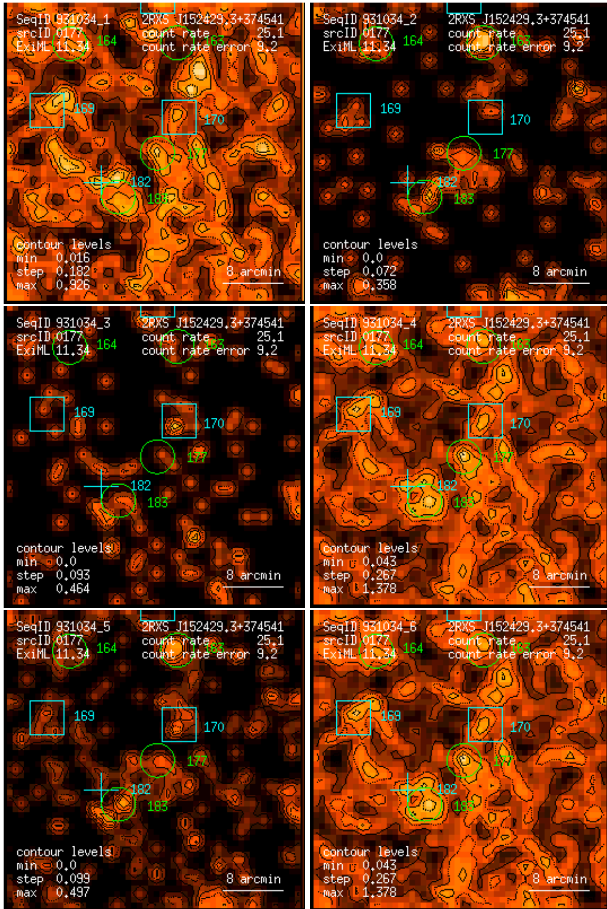
Figure 177: RASS 931034: detection 0177: band rate images, Gaussian filter: (1) PSPC channels 11 – 41, (2) 52 – 90, (3) 91 – 201, (4) 11 – 235, (5) 52 – 201, (6) 11 – 201. Broad band rates in counts/ks. Band rate contour levels in counts/ks/arcmin 2 .
