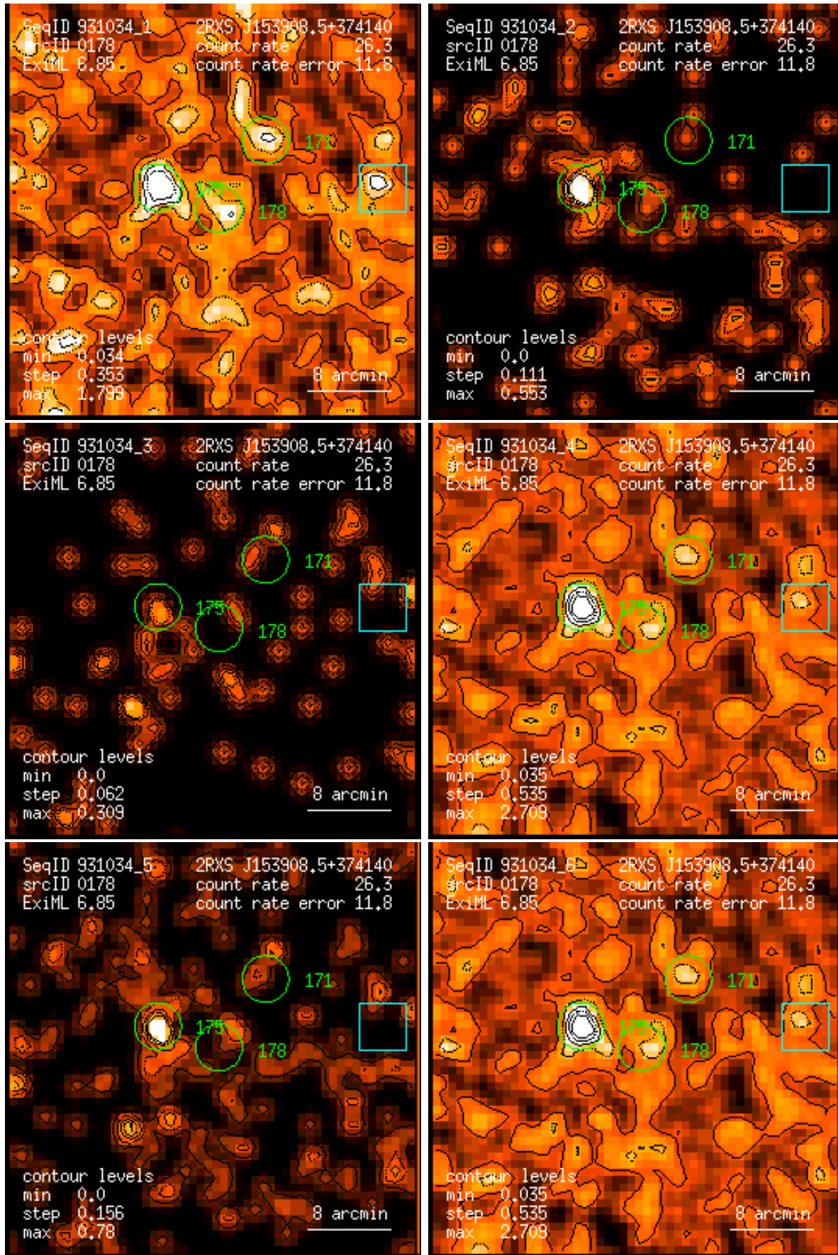
Figure 178: RASS 931034: detection 0178: band rate images, Gaussian filter: (1) PSPC channels 11 – 41, (2) 52 – 90, (3) 91 – 201, (4) 11 – 235, (5) 52 – 201, (6) 11 – 201. Broad band rates in counts/ks. Band rate contour levels in counts/ks/arcmin 2 .
