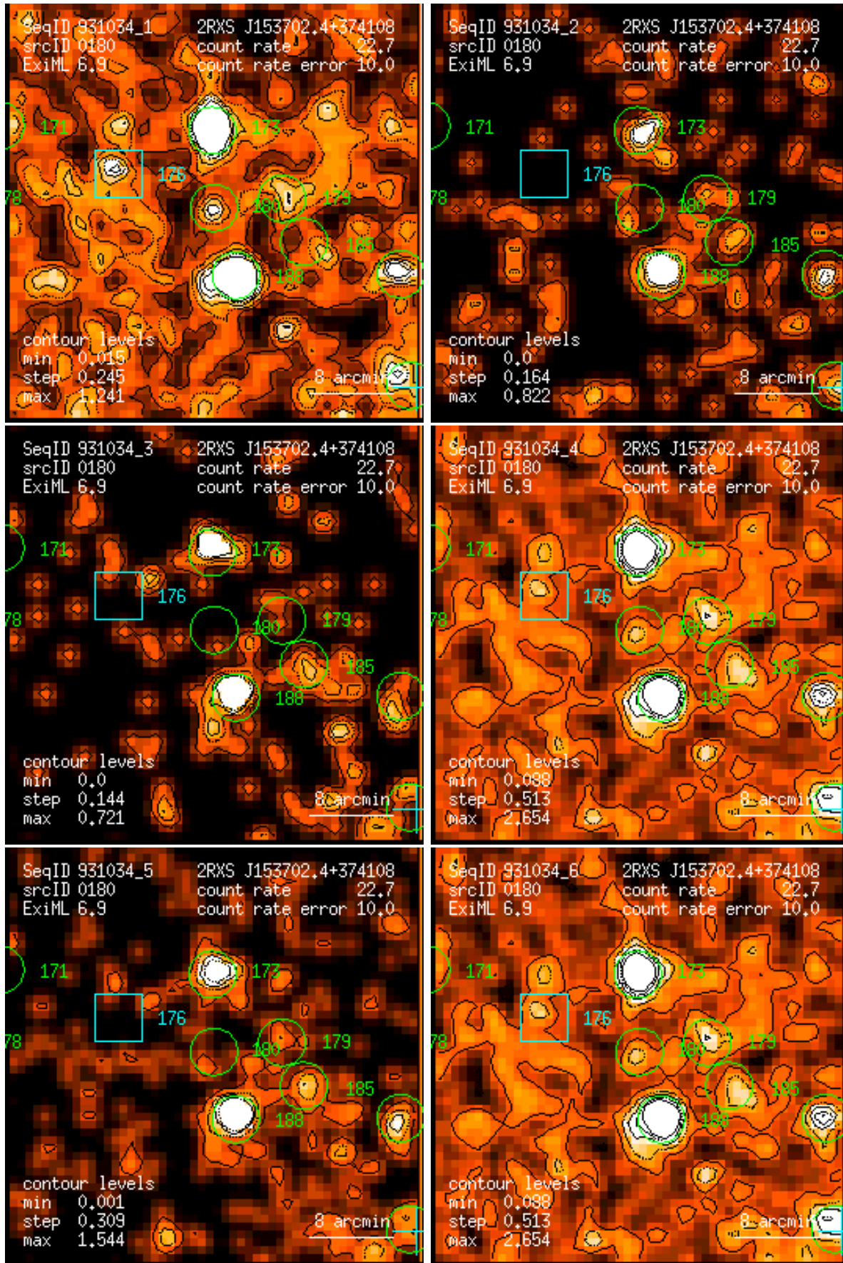
Figure 180: RASS 931034: detection 0180: band rate images, Gaussian filter: (1) PSPC channels 11 – 41, (2) 52 – 90, (3) 91 – 201, (4) 11 – 235, (5) 52 – 201, (6) 11 – 201. Broad band rates in counts/ks. Band rate contour levels in counts/ks/arcmin 2 .
