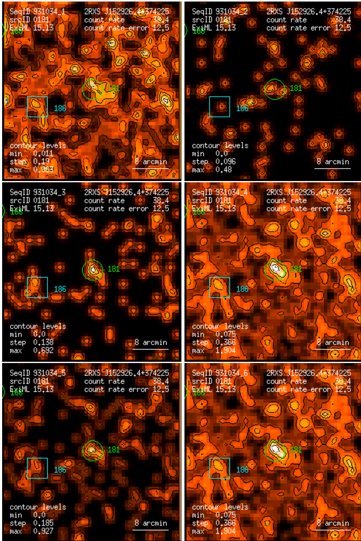
Figure 181: RASS 931034: detection 0181: band rate images, Gaussian filter: (1) PSPC channels 11 – 41, (2) 52 – 90, (3) 91 – 201, (4) 11 – 235, (5) 52 – 201, (6) 11 – 201. Broad band rates in counts/ks. Band rate contour levels in counts/ks/arcmin 2 .
