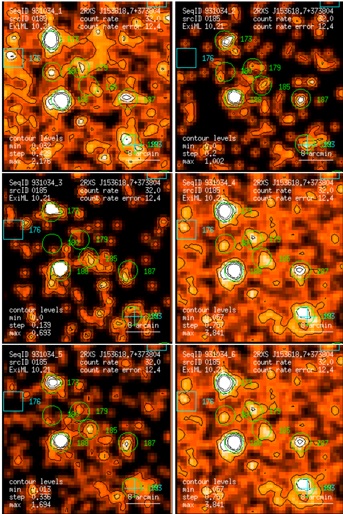
Figure 185: RASS 931034: detection 0185: band rate images, Gaussian filter: (1) PSPC channels 11 – 41, (2) 52 – 90, (3) 91 – 201, (4) 11 – 235, (5) 52 – 201, (6) 11 – 201. Broad band rates in counts/ks. Band rate contour levels in counts/ks/arcmin 2 .
