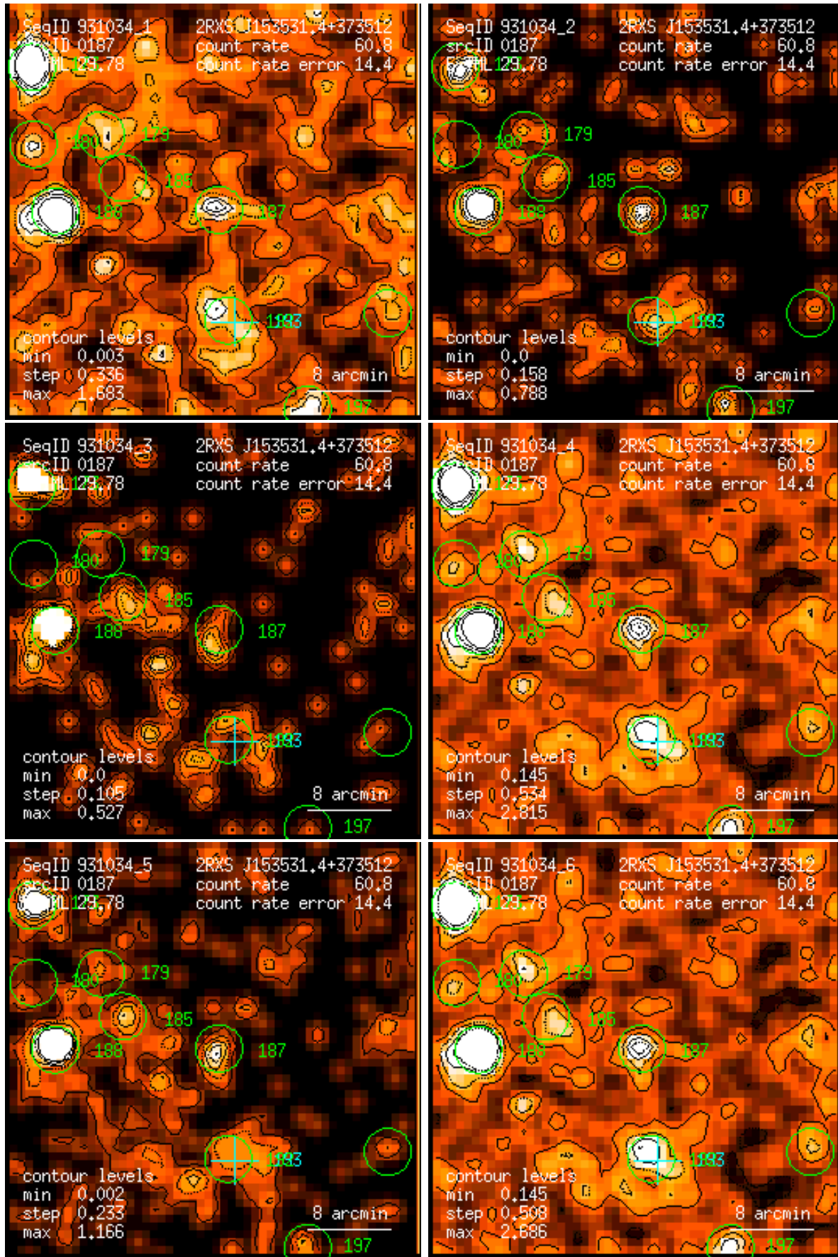
Figure 187: RASS 931034: detection 0187: band rate images, Gaussian filter: (1) PSPC channels 11 – 41, (2) 52 – 90, (3) 91 – 201, (4) 11 – 235, (5) 52 – 201, (6) 11 – 201. Broad band rates in counts/ks. Band rate contour levels in counts/ks/arcmin 2 .
