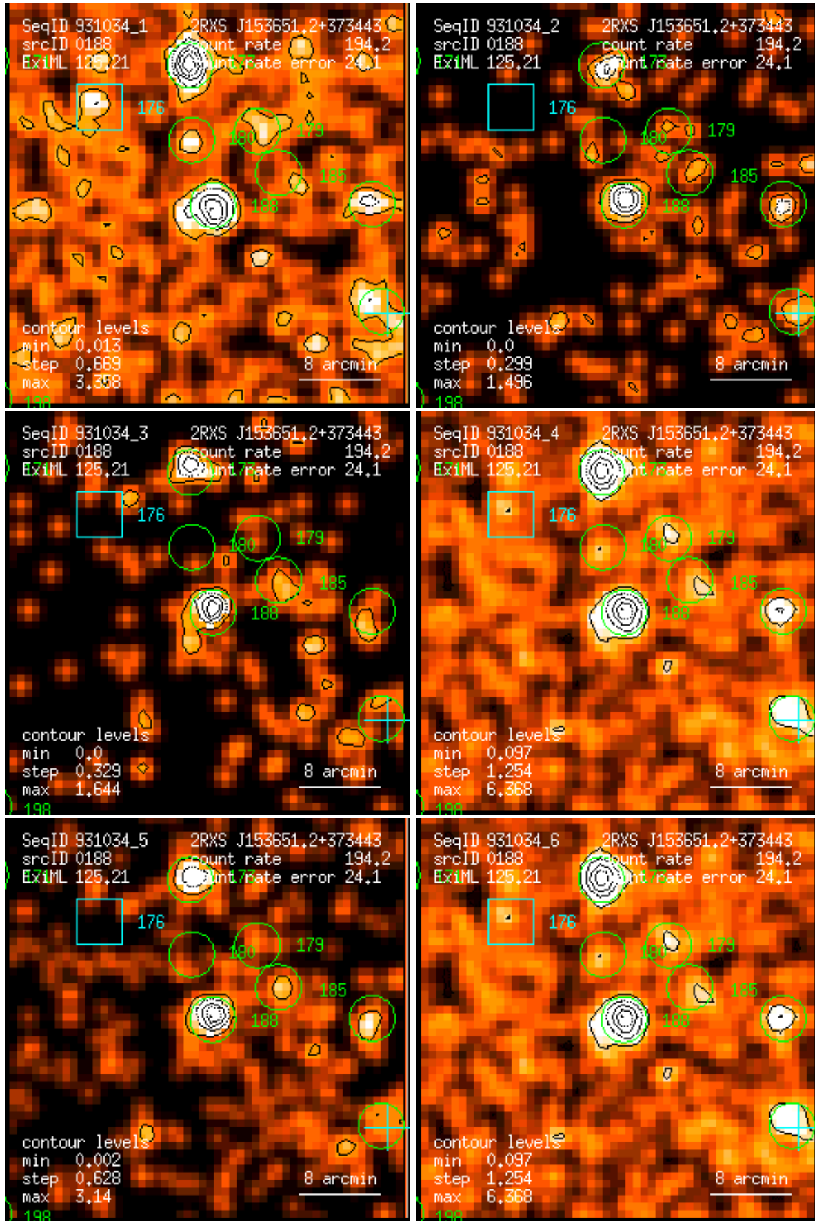
Figure 188: RASS 931034: detection 0188: band rate images, Gaussian filter: (1) PSPC channels 11 – 41, (2) 52 – 90, (3) 91 – 201, (4) 11 – 235, (5) 52 – 201, (6) 11 – 201. Broad band rates in counts/ks. Band rate contour levels in counts/ks/arcmin 2 .
