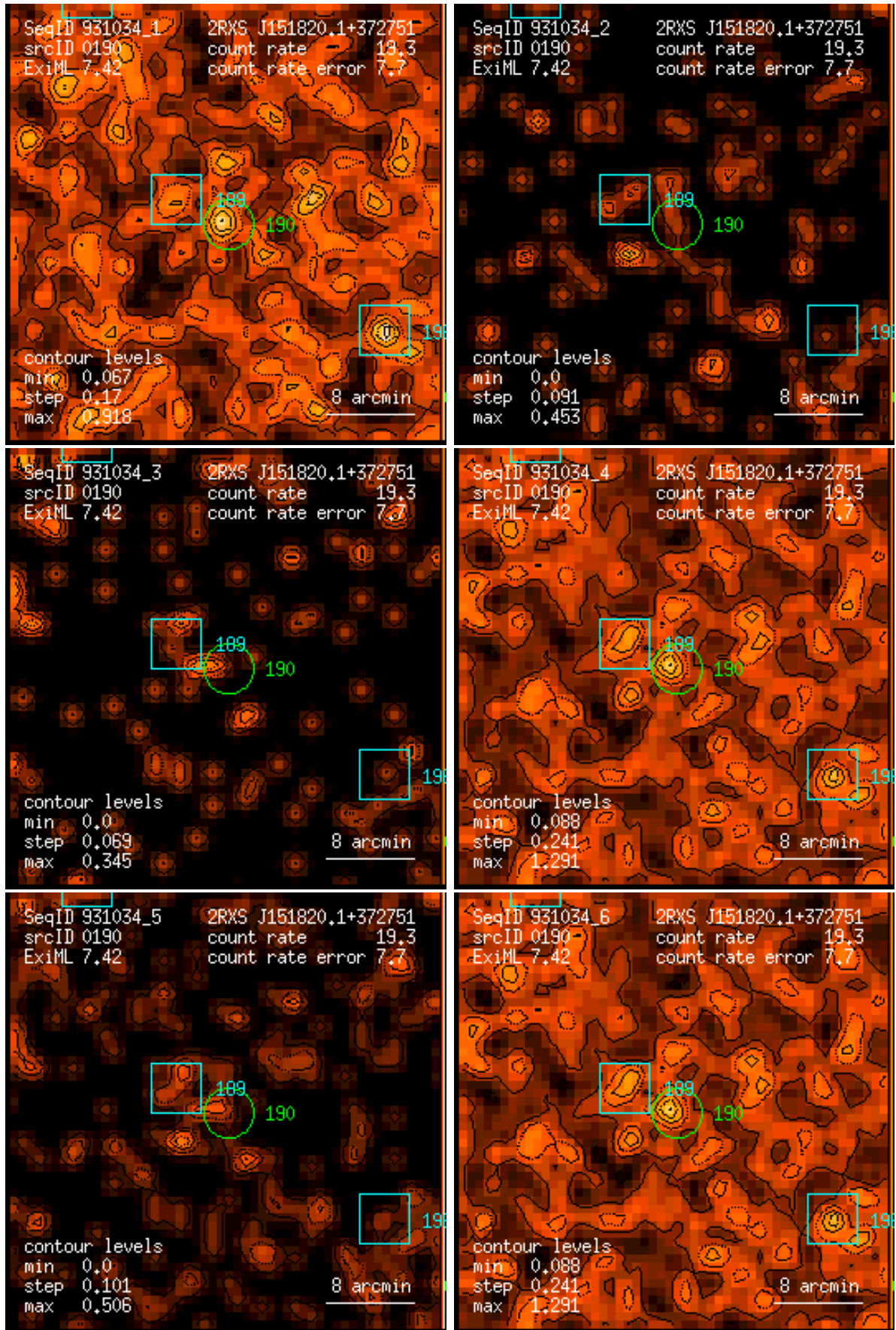
Figure 190: RASS 931034: detection 0190: band rate images, Gaussian filter: (1) PSPC channels 11 – 41, (2) 52 – 90, (3) 91 – 201, (4) 11 – 235, (5) 52 – 201, (6) 11 – 201. Broad band rates in counts/ks. Band rate contour levels in counts/ks/arcmin 2 .
