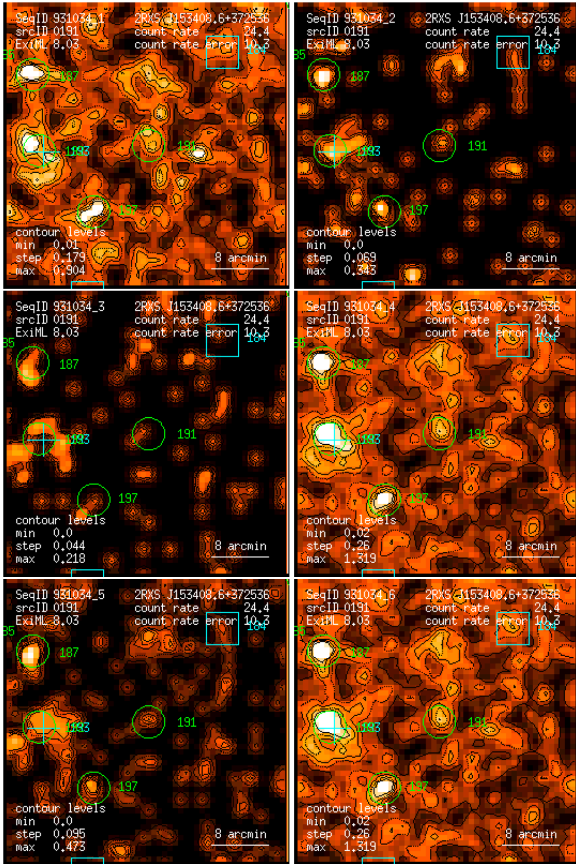
Figure 191: RASS 931034: detection 0191: band rate images, Gaussian filter: (1) PSPC channels 11 – 41, (2) 52 – 90, (3) 91 – 201, (4) 11 – 235, (5) 52 – 201, (6) 11 – 201. Broad band rates in counts/ks. Band rate contour levels in counts/ks/arcmin 2 .
