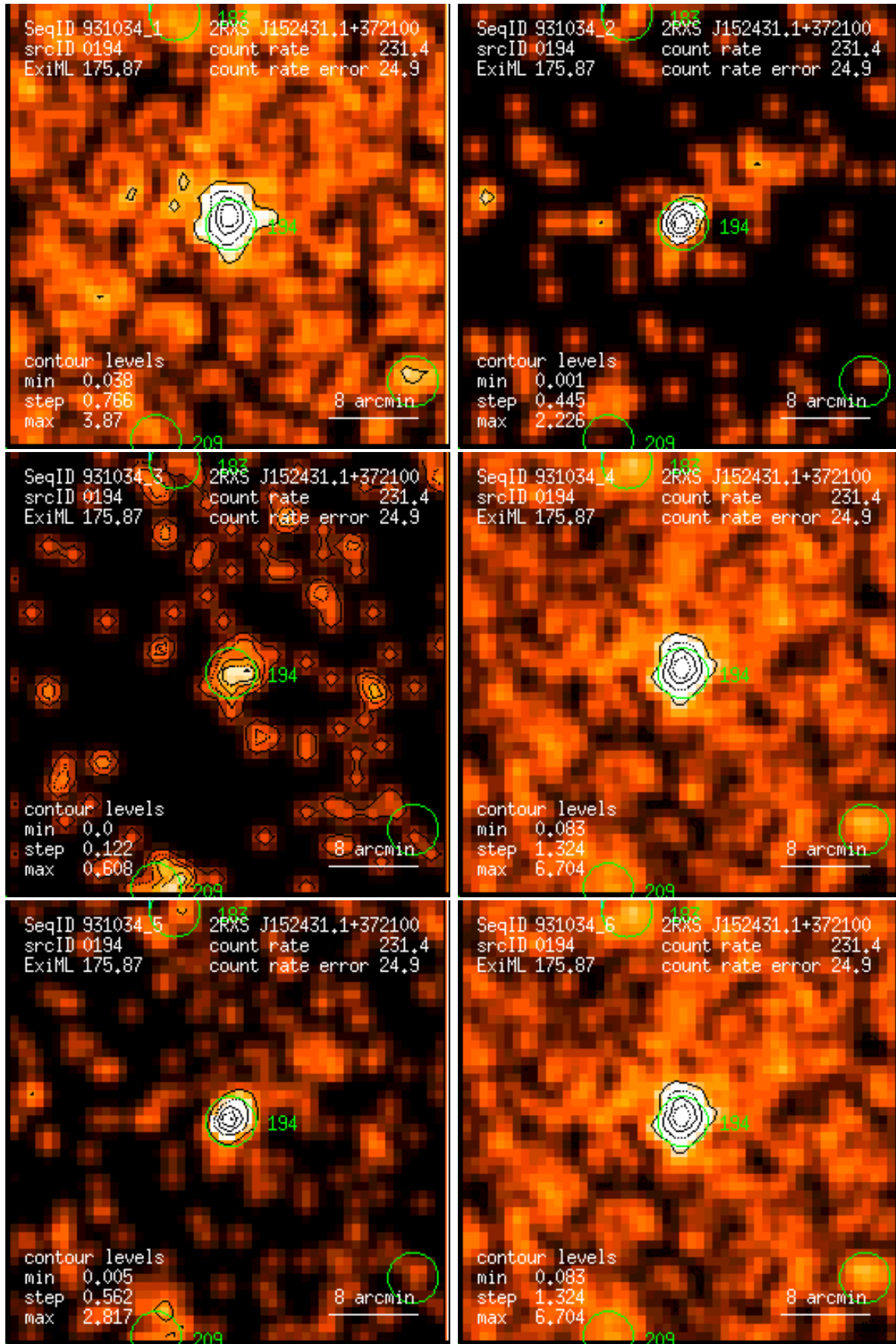
Figure 194: RASS 931034: detection 0194: band rate images, Gaussian filter: (1) PSPC channels 11 – 41, (2) 52 – 90, (3) 91 – 201, (4) 11 – 235, (5) 52 – 201, (6) 11 – 201. Broad band rates in counts/ks. Band rate contour levels in counts/ks/arcmin 2 .
