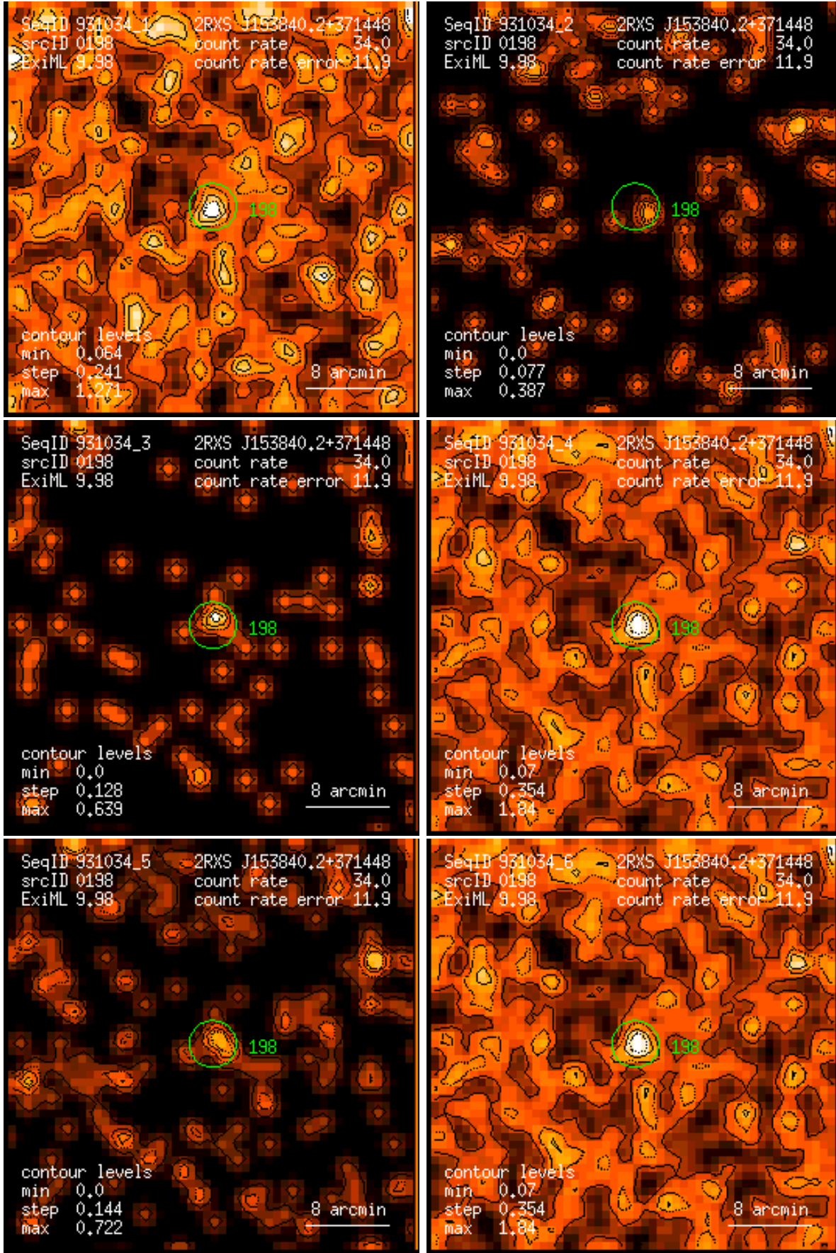
Figure 198: RASS 931034: detection 0198: band rate images, Gaussian filter: (1) PSPC channels 11 – 41, (2) 52 – 90, (3) 91 – 201, (4) 11 – 235, (5) 52 – 201, (6) 11 – 201. Broad band rates in counts/ks. Band rate contour levels in counts/ks/arcmin 2 .
