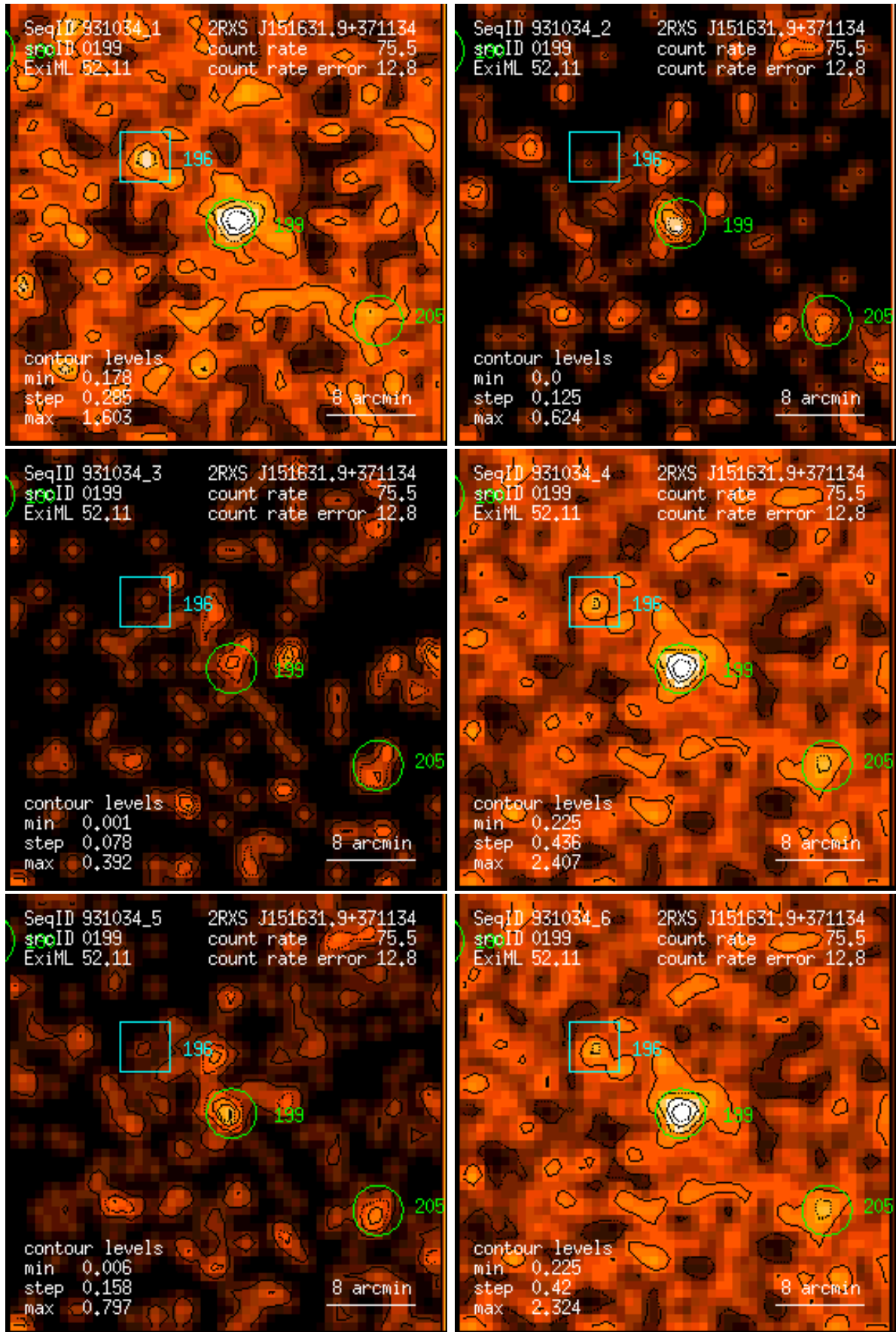
Figure 199: RASS 931034: detection 0199: band rate images, Gaussian filter: (1) PSPC channels 11 – 41, (2) 52 – 90, (3) 91 – 201, (4) 11 – 235, (5) 52 – 201, (6) 11 – 201. Broad band rates in counts/ks. Band rate contour levels in counts/ks/arcmin 2 .
