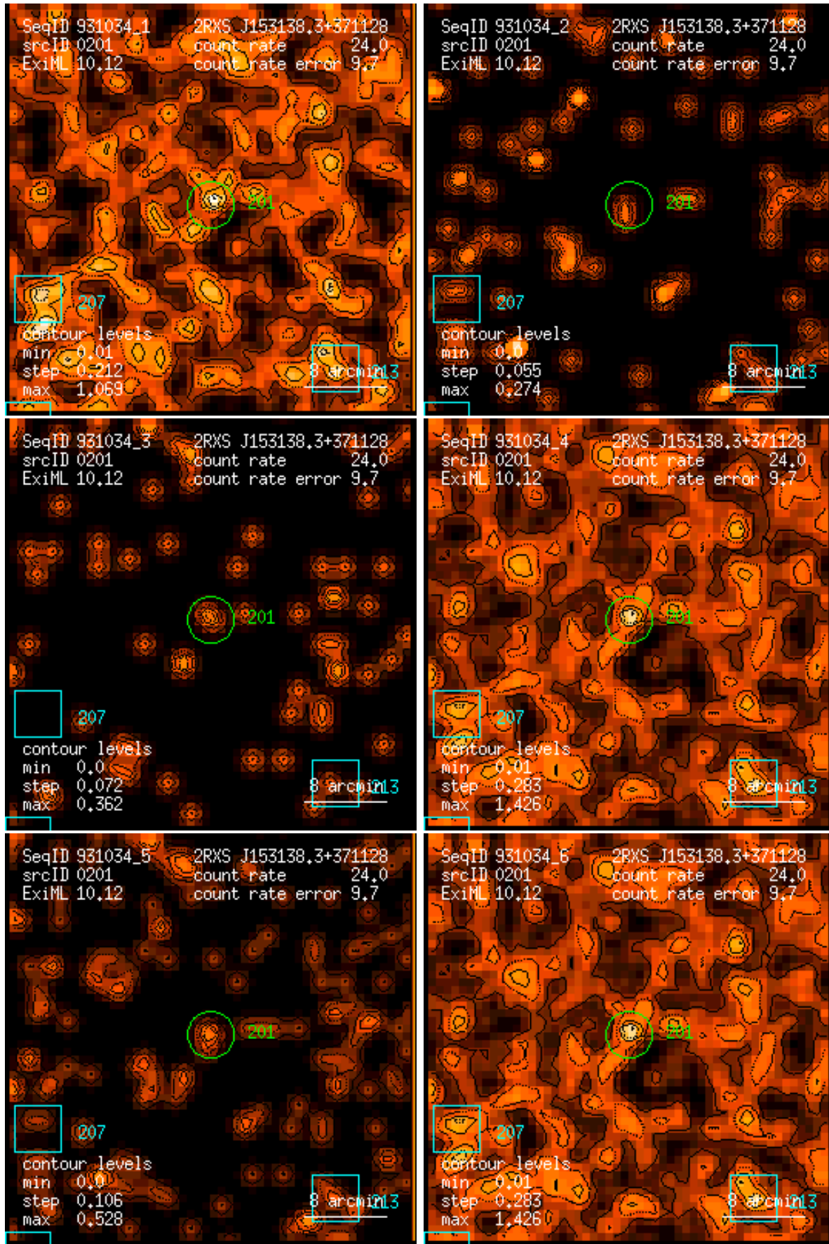
Figure 201: RASS 931034: detection 0201: band rate images, Gaussian filter: (1) PSPC channels 11 – 41, (2) 52 – 90, (3) 91 – 201, (4) 11 – 235, (5) 52 – 201, (6) 11 – 201. Broad band rates in counts/ks. Band rate contour levels in counts/ks/arcmin 2 .
