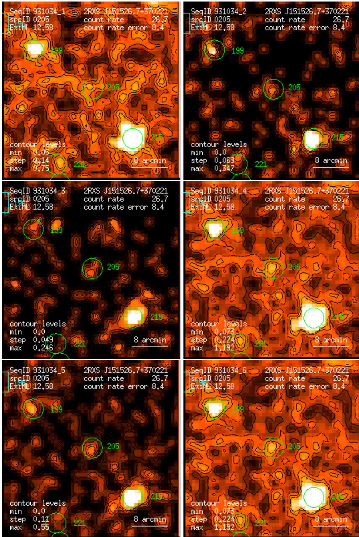
Figure 205: RASS 931034: detection 0205: band rate images, Gaussian filter: (1) PSPC channels 11 – 41, (2) 52 – 90, (3) 91 – 201, (4) 11 – 235, (5) 52 – 201, (6) 11 – 201. Broad band rates in counts/ks. Band rate contour levels in counts/ks/arcmin 2 .
