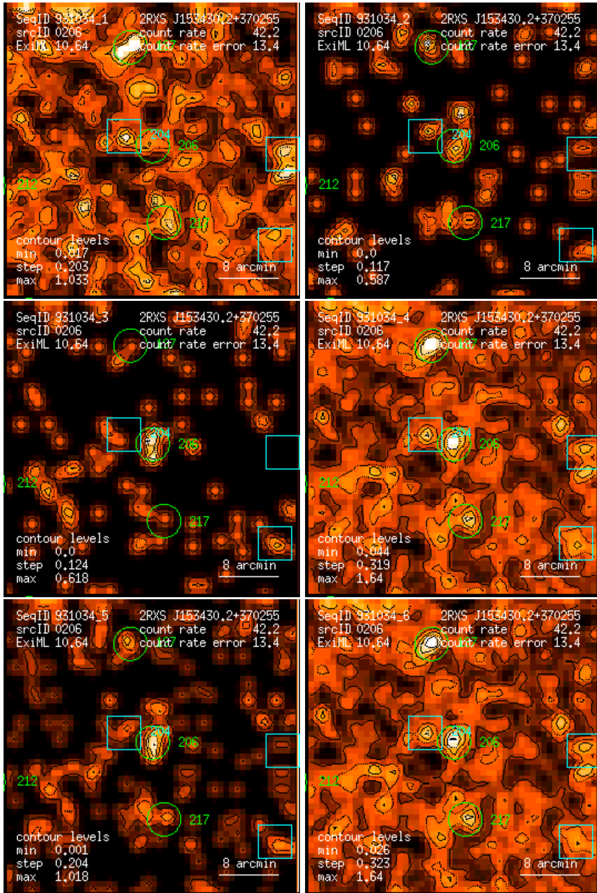
Figure 206: RASS 931034: detection 0206: band rate images, Gaussian filter: (1) PSPC channels 11 – 41, (2) 52 – 90, (3) 91 – 201, (4) 11 – 235, (5) 52 – 201, (6) 11 – 201. Broad band rates in counts/ks. Band rate contour levels in counts/ks/arcmin 2 .
