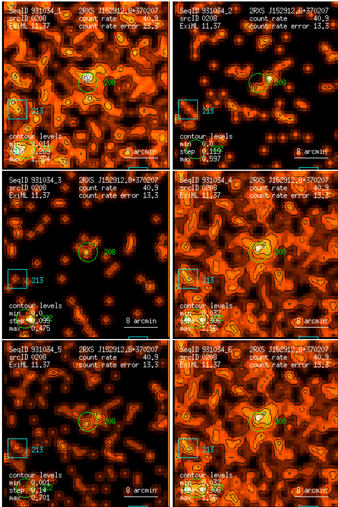
Figure 208: RASS 931034: detection 0208: band rate images, Gaussian filter: (1) PSPC channels 11 – 41, (2) 52 – 90, (3) 91 – 201, (4) 11 – 235, (5) 52 – 201, (6) 11 – 201. Broad band rates in counts/ks. Band rate contour levels in counts/ks/arcmin 2 .
