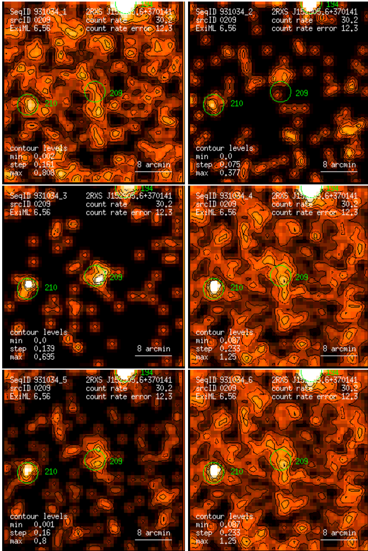
Figure 209: RASS 931034: detection 0209: band rate images, Gaussian filter: (1) PSPC channels 11 – 41, (2) 52 – 90, (3) 91 – 201, (4) 11 – 235, (5) 52 – 201, (6) 11 – 201. Broad band rates in counts/ks. Band rate contour levels in counts/ks/arcmin 2 .
