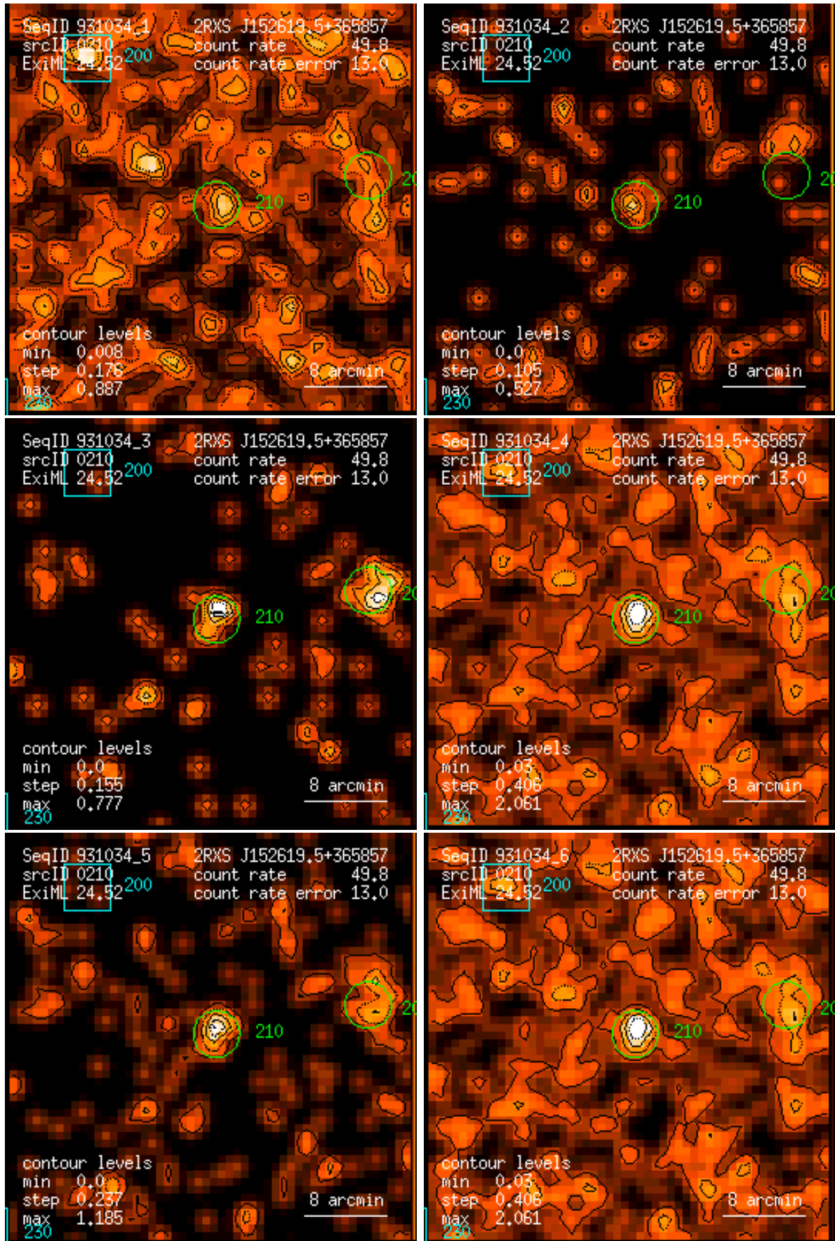
Figure 210: RASS 931034: detection 0210: band rate images, Gaussian filter: (1) PSPC channels 11 – 41, (2) 52 – 90, (3) 91 – 201, (4) 11 – 235, (5) 52 – 201, (6) 11 – 201. Broad band rates in counts/ks. Band rate contour levels in counts/ks/arcmin 2 .
