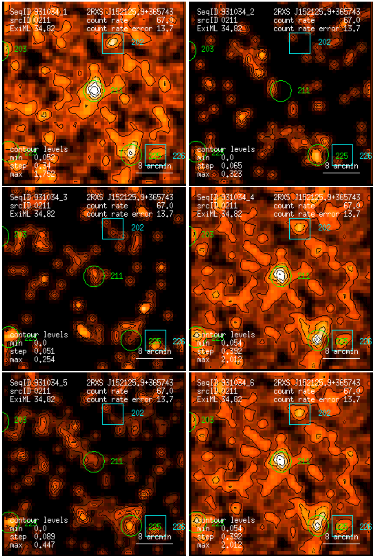
Figure 211: RASS 931034: detection 0211: band rate images, Gaussian filter: (1) PSPC channels 11 – 41, (2) 52 – 90, (3) 91 – 201, (4) 11 – 235, (5) 52 – 201, (6) 11 – 201. Broad band rates in counts/ks. Band rate contour levels in counts/ks/arcmin 2 .
