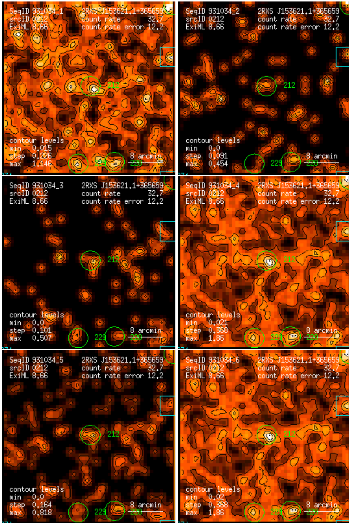
Figure 212: RASS 931034: detection 0212: band rate images, Gaussian filter: (1) PSPC channels 11 – 41, (2) 52 – 90, (3) 91 – 201, (4) 11 – 235, (5) 52 – 201, (6) 11 – 201. Broad band rates in counts/ks. Band rate contour levels in counts/ks/arcmin 2 .
