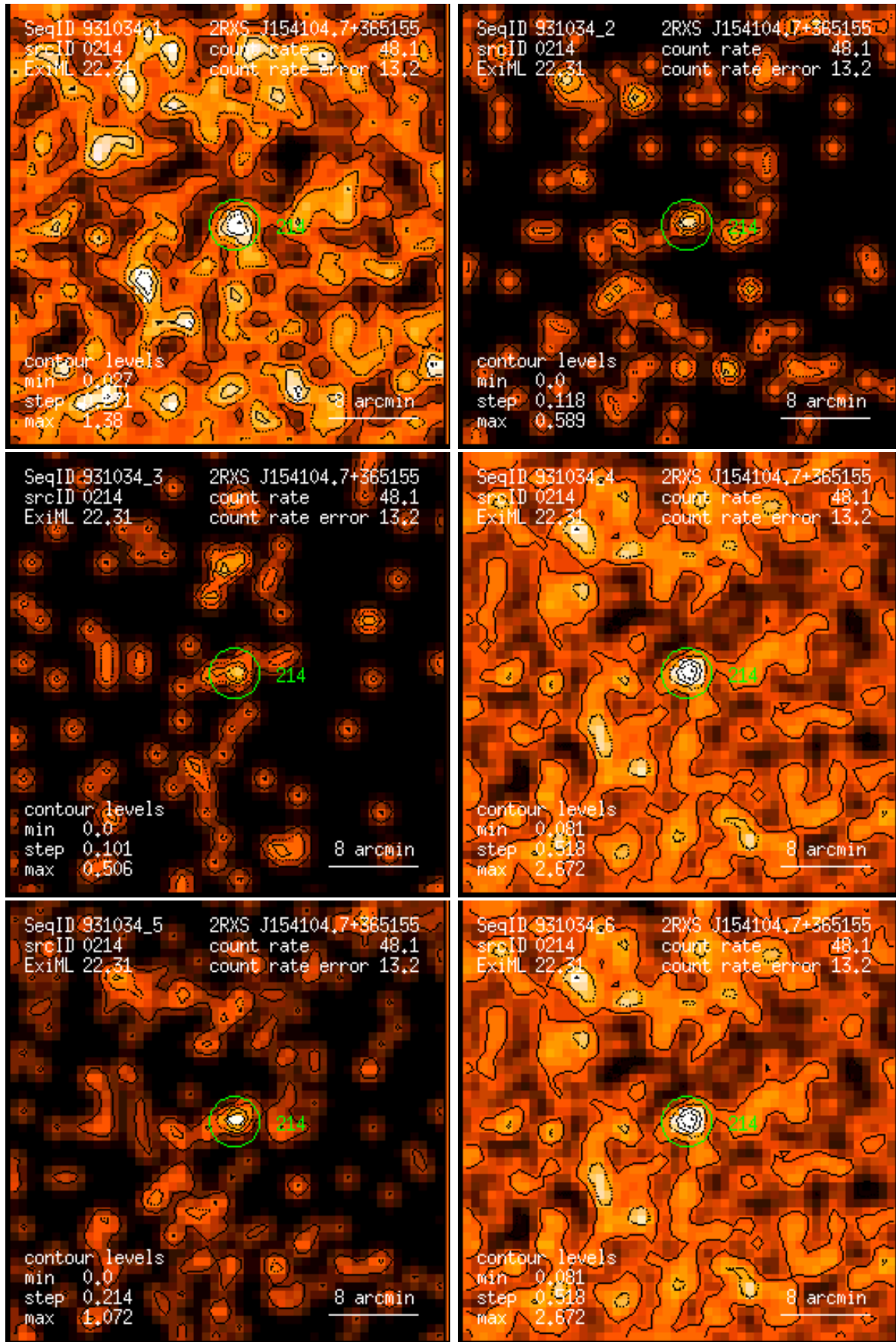
Figure 214: RASS 931034: detection 0214: band rate images, Gaussian filter: (1) PSPC channels 11 – 41, (2) 52 – 90, (3) 91 – 201, (4) 11 – 235, (5) 52 – 201, (6) 11 – 201. Broad band rates in counts/ks. Band rate contour levels in counts/ks/arcmin 2 .
