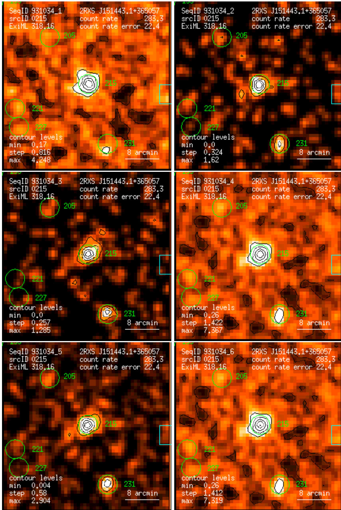
Figure 215: RASS 931034: detection 0215: band rate images, Gaussian filter: (1) PSPC channels 11 – 41, (2) 52 – 90, (3) 91 – 201, (4) 11 – 235, (5) 52 – 201, (6) 11 – 201. Broad band rates in counts/ks. Band rate contour levels in counts/ks/arcmin 2 .
