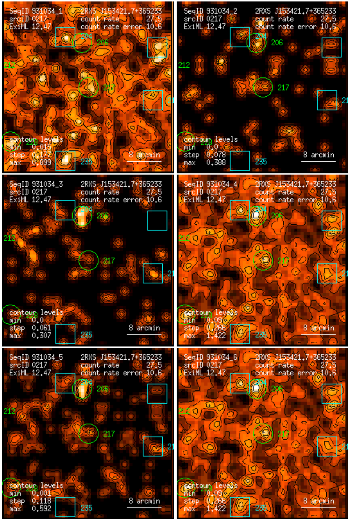
Figure 217: RASS 931034: detection 0217: band rate images, Gaussian filter: (1) PSPC channels 11 – 41, (2) 52 – 90, (3) 91 – 201, (4) 11 – 235, (5) 52 – 201, (6) 11 – 201. Broad band rates in counts/ks. Band rate contour levels in counts/ks/arcmin 2 .
