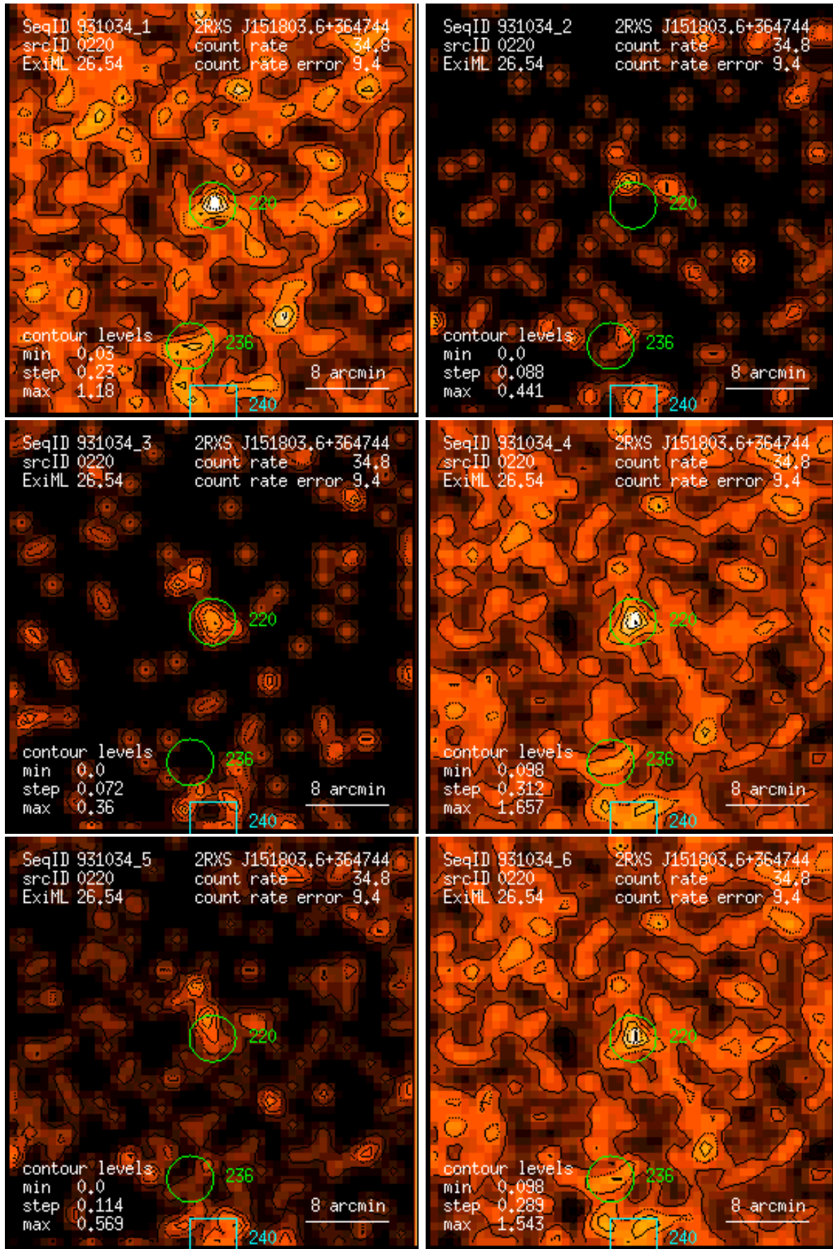
Figure 220: RASS 931034: detection 0220: band rate images, Gaussian filter: (1) PSPC channels 11 – 41, (2) 52 – 90, (3) 91 – 201, (4) 11 – 235, (5) 52 – 201, (6) 11 – 201. Broad band rates in counts/ks. Band rate contour levels in counts/ks/arcmin 2 .
