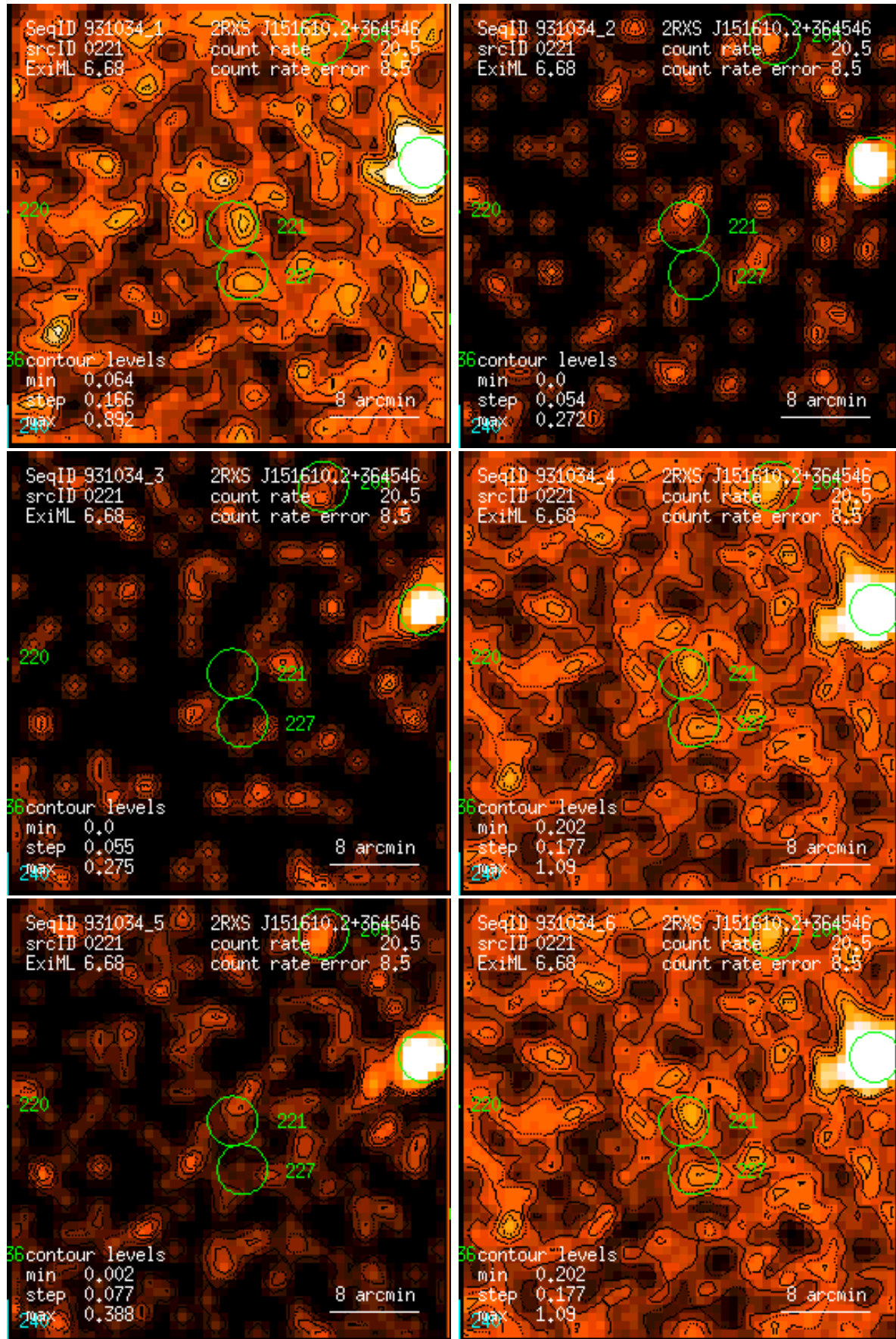
Figure 221: RASS 931034: detection 0221: band rate images, Gaussian filter: (1) PSPC channels 11 – 41, (2) 52 – 90, (3) 91 – 201, (4) 11 – 235, (5) 52 – 201, (6) 11 – 201. Broad band rates in counts/ks. Band rate contour levels in counts/ks/arcmin 2 .
