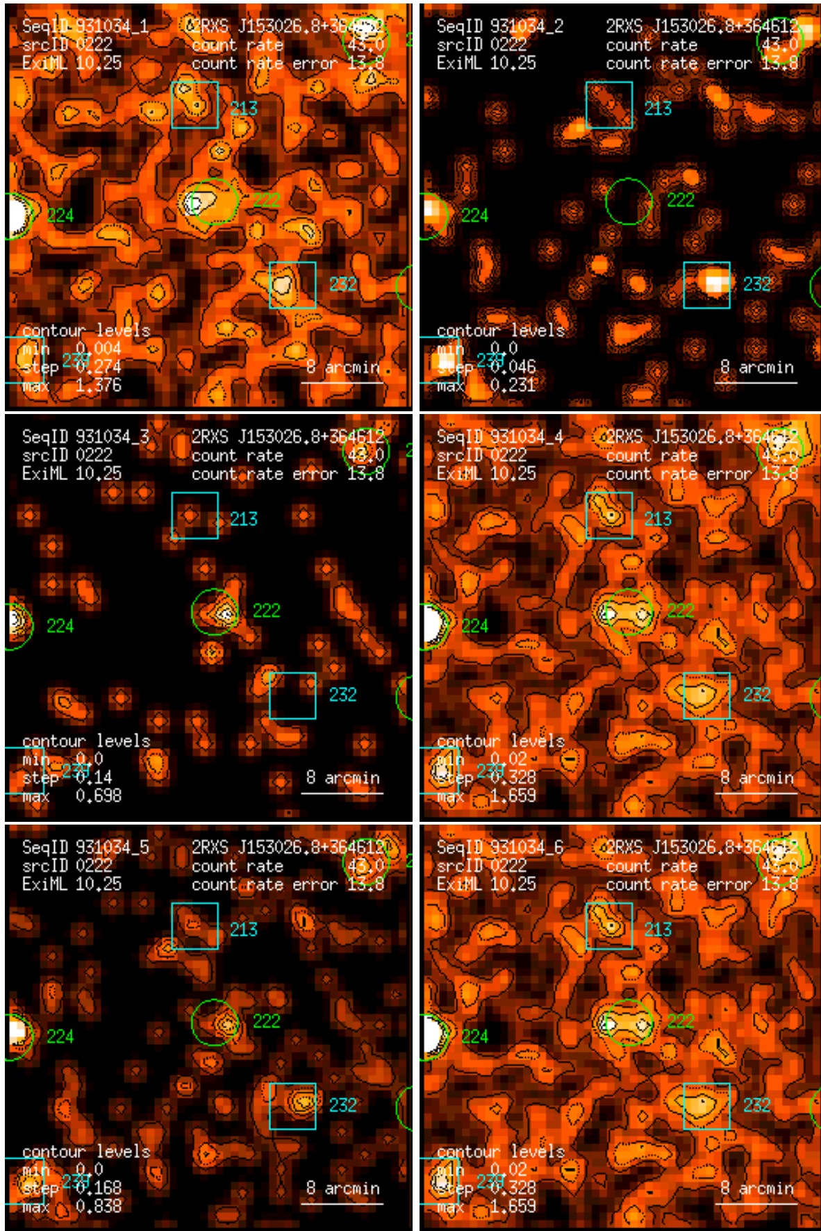
Figure 222: RASS 931034: detection 0222: band rate images, Gaussian filter: (1) PSPC channels 11 – 41, (2) 52 – 90, (3) 91 – 201, (4) 11 – 235, (5) 52 – 201, (6) 11 – 201. Broad band rates in counts/ks. Band rate contour levels in counts/ks/arcmin 2 .
