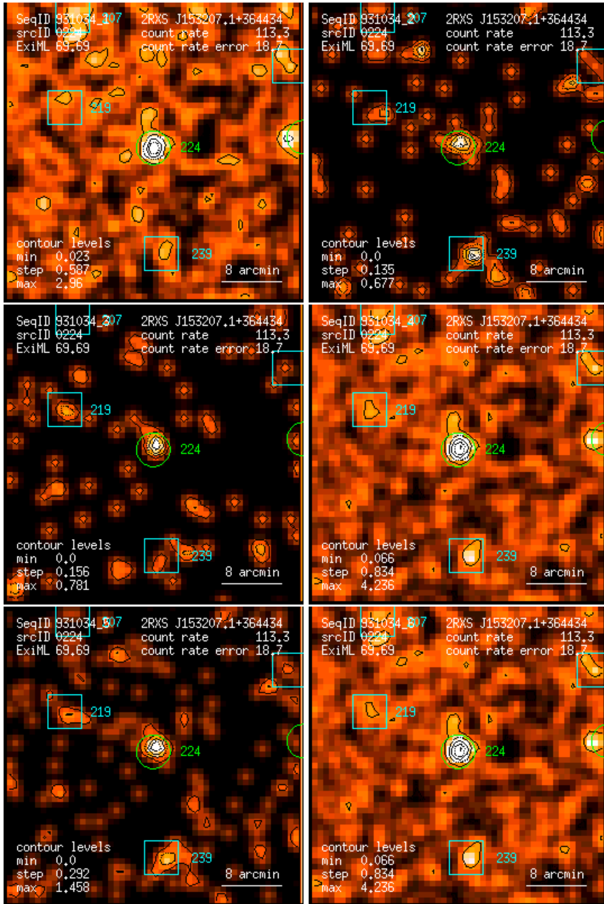
Figure 224: RASS 931034: detection 0224: band rate images, Gaussian filter: (1) PSPC channels 11 – 41, (2) 52 – 90, (3) 91 – 201, (4) 11 – 235, (5) 52 – 201, (6) 11 – 201. Broad band rates in counts/ks. Band rate contour levels in counts/ks/arcmin 2 .
