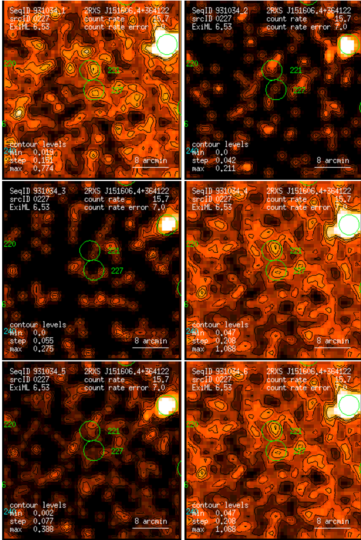
Figure 227: RASS 931034: detection 0227: band rate images, Gaussian filter: (1) PSPC channels 11 – 41, (2) 52 – 90, (3) 91 – 201, (4) 11 – 235, (5) 52 – 201, (6) 11 – 201. Broad band rates in counts/ks. Band rate contour levels in counts/ks/arcmin 2 .
