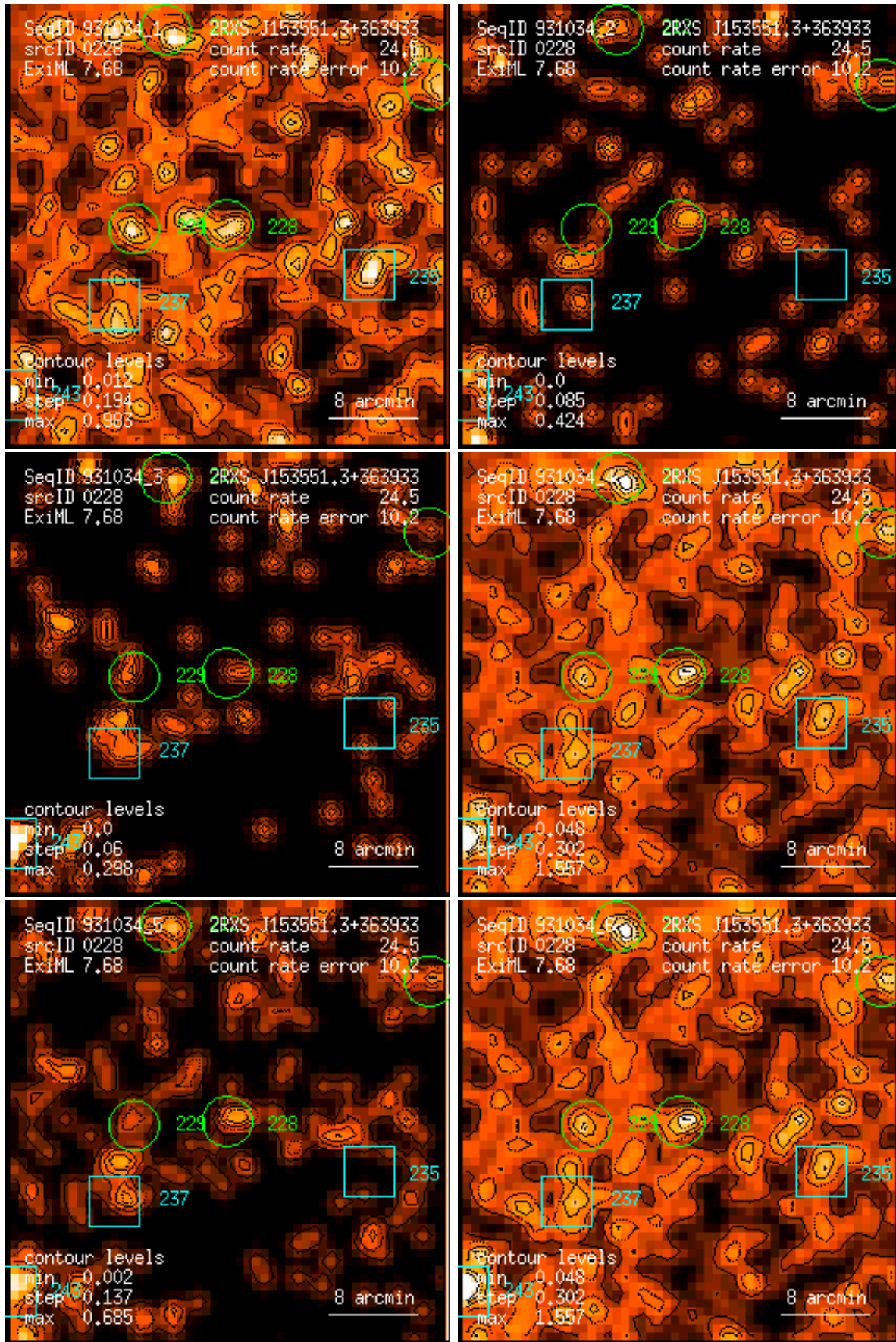
Figure 228: RASS 931034: detection 0228: band rate images, Gaussian filter: (1) PSPC channels 11 – 41, (2) 52 – 90, (3) 91 – 201, (4) 11 – 235, (5) 52 – 201, (6) 11 – 201. Broad band rates in counts/ks. Band rate contour levels in counts/ks/arcmin 2 .
