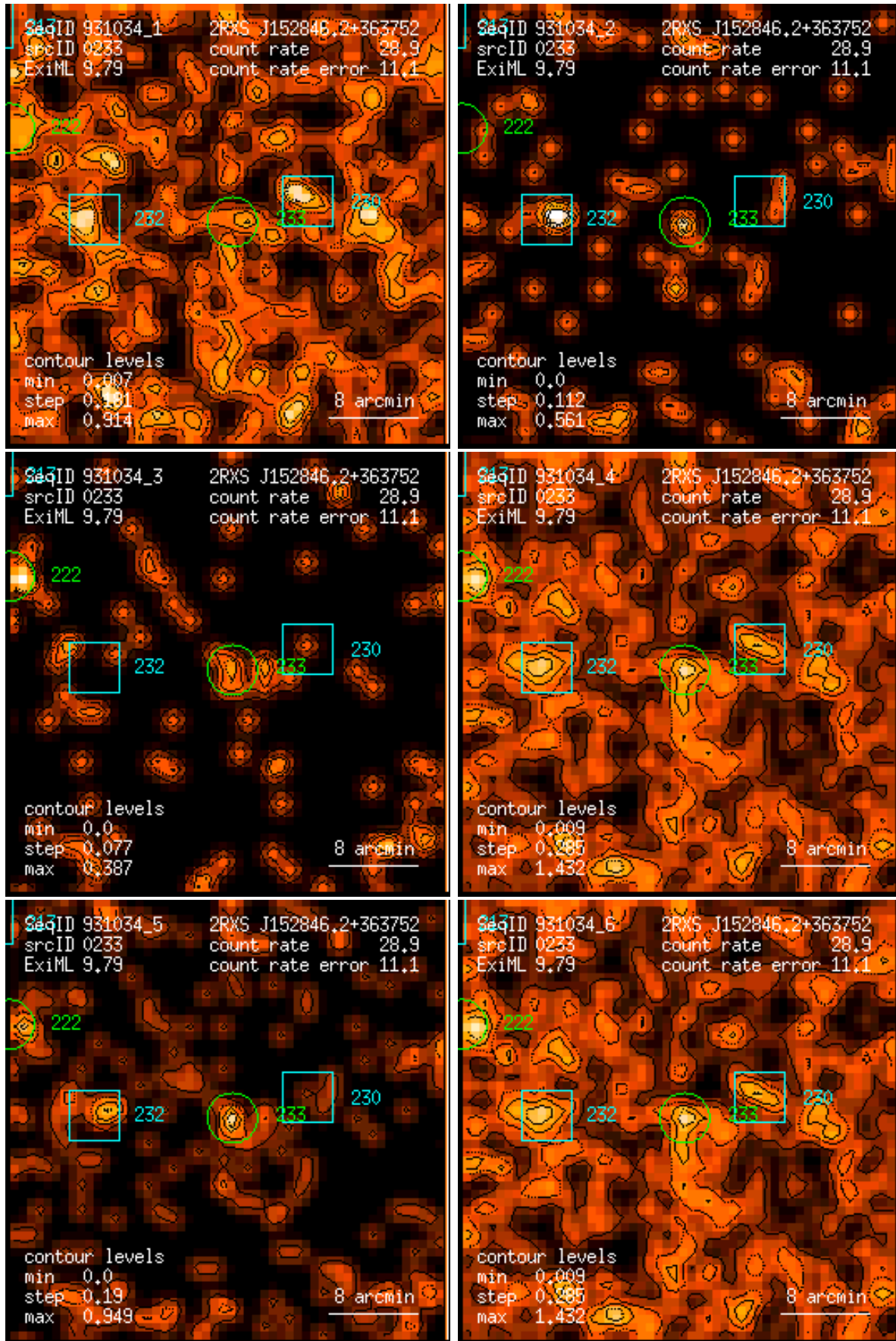
Figure 233: RASS 931034: detection 0233: band rate images, Gaussian filter: (1) PSPC channels 11 – 41, (2) 52 – 90, (3) 91 – 201, (4) 11 – 235, (5) 52 – 201, (6) 11 – 201. Broad band rates in counts/ks. Band rate contour levels in counts/ks/arcmin 2 .
