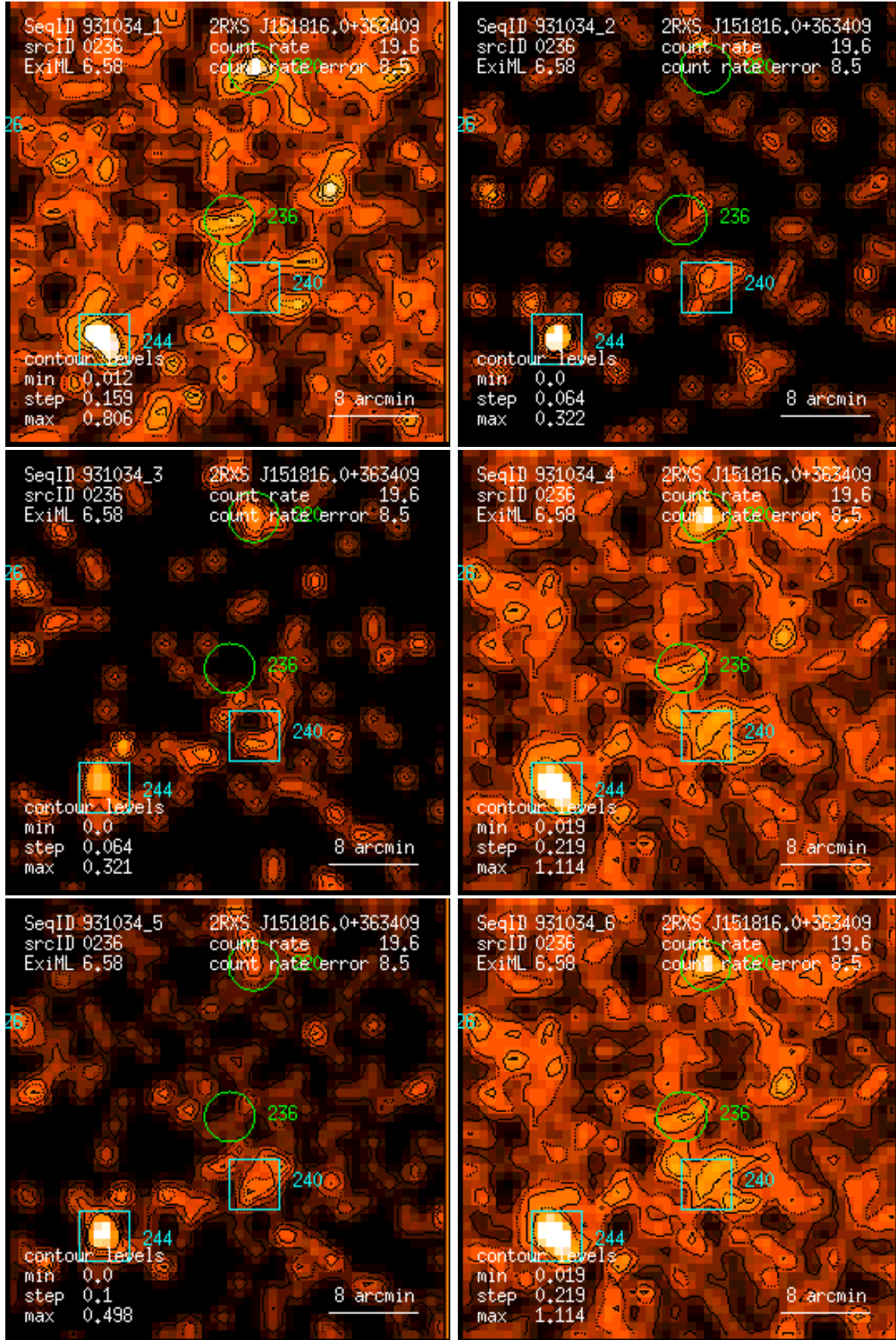
Figure 236: RASS 931034: detection 0236: band rate images, Gaussian filter: (1) PSPC channels 11 – 41, (2) 52 – 90, (3) 91 – 201, (4) 11 – 235, (5) 52 – 201, (6) 11 – 201. Broad band rates in counts/ks. Band rate contour levels in counts/ks/arcmin 2 .
