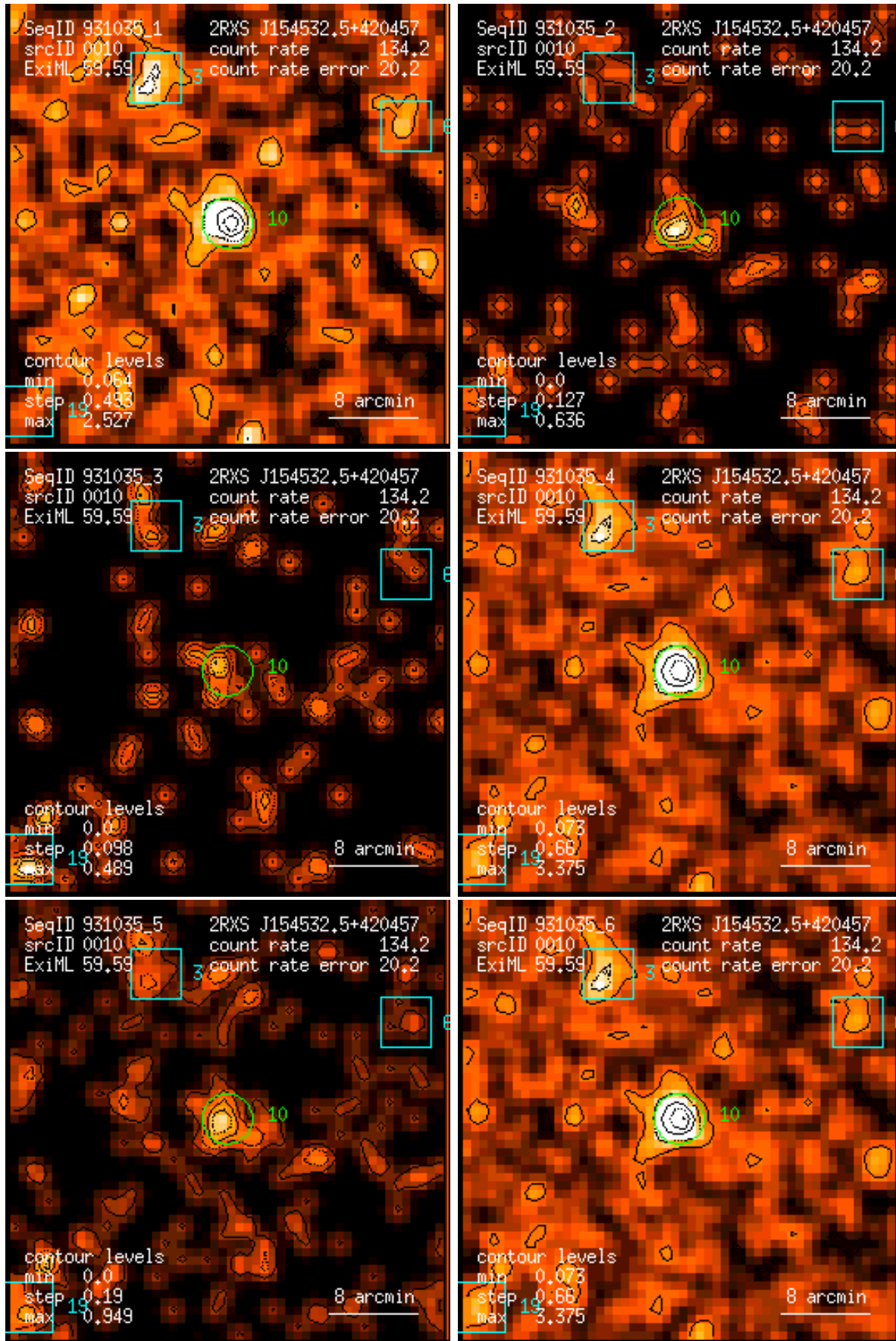
Figure 10: RASS 931035: detection 0010: band rate images, Gaussian filter: (1) PSPC channels 11 – 41, (2) 52 – 90, (3) 91 – 201, (4) 11 – 235, (5) 52 – 201, (6) 11 – 201. Broad band rates in counts/ks. Band rate contour levels in counts/ks/arcmin 2 .
