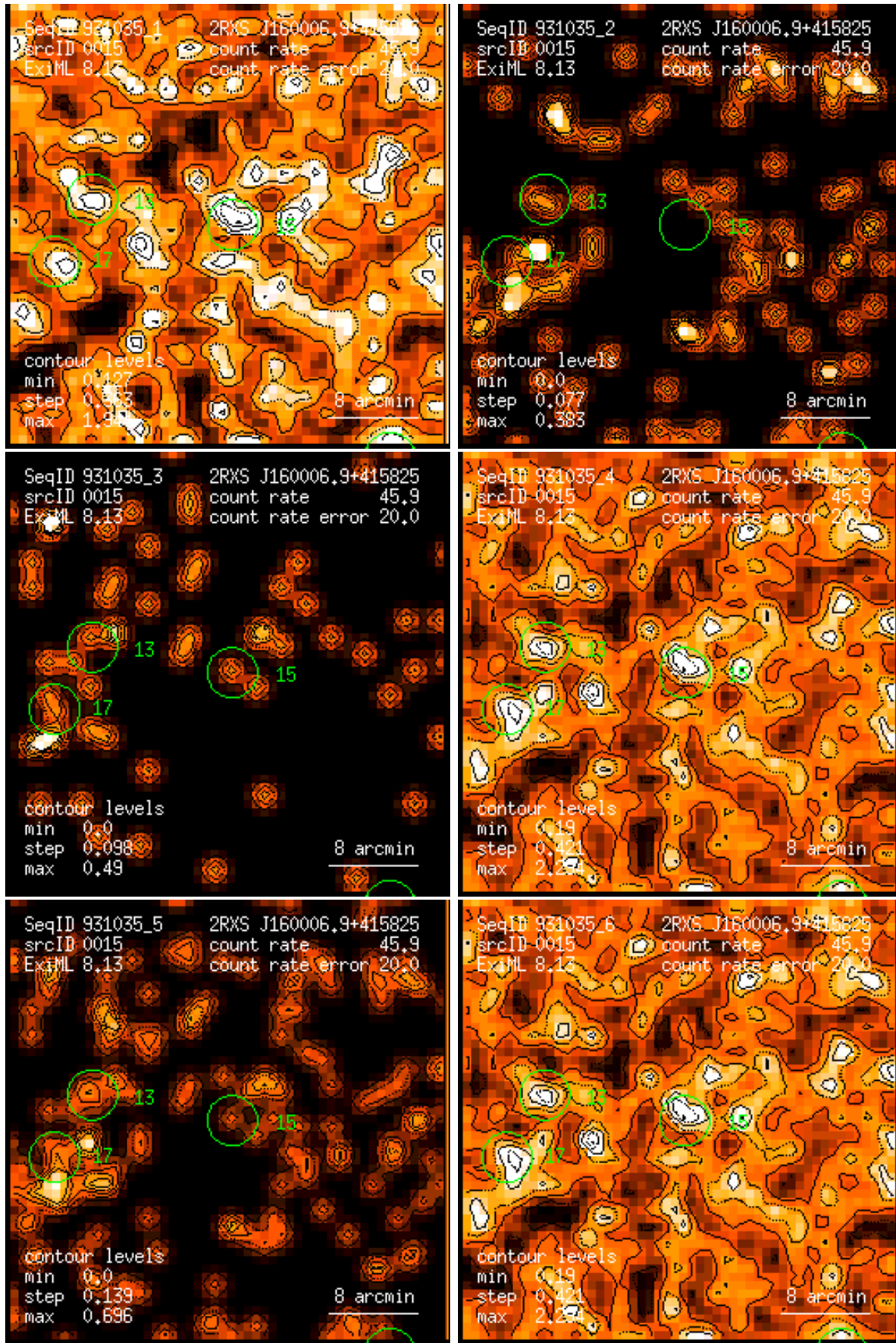
Figure 15: RASS 931035: detection 0015: band rate images, Gaussian filter: (1) PSPC channels 11 – 41, (2) 52 – 90, (3) 91 – 201, (4) 11 – 235, (5) 52 – 201, (6) 11 – 201. Broad band rates in counts/ks. Band rate contour levels in counts/ks/arcmin 2 .
