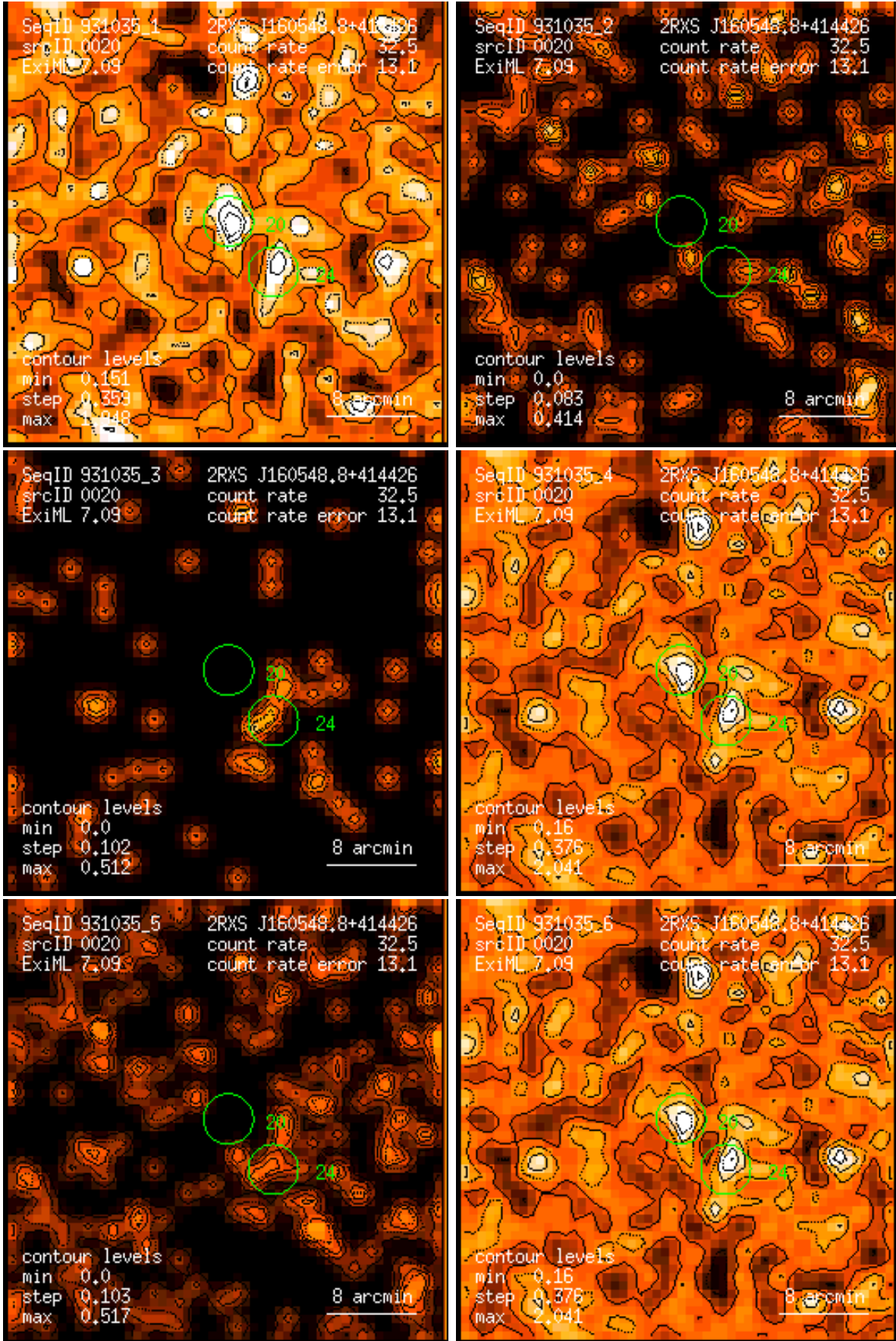
Figure 20: RASS 931035: detection 0020: band rate images, Gaussian filter: (1) PSPC channels 11 – 41, (2) 52 – 90, (3) 91 – 201, (4) 11 – 235, (5) 52 – 201, (6) 11 – 201. Broad band rates in counts/ks. Band rate contour levels in counts/ks/arcmin 2 .
