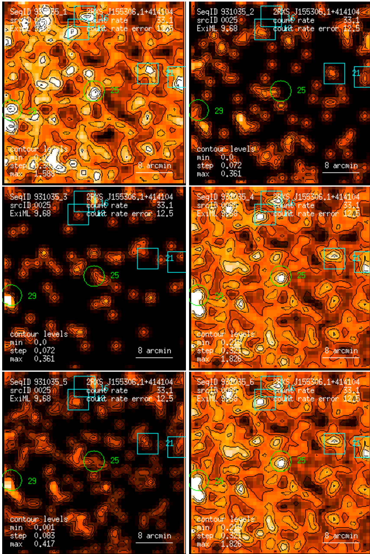
Figure 25: RASS 931035: detection 0025: band rate images, Gaussian filter: (1) PSPC channels 11 – 41, (2) 52 – 90, (3) 91 – 201, (4) 11 – 235, (5) 52 – 201, (6) 11 – 201. Broad band rates in counts/ks. Band rate contour levels in counts/ks/arcmin 2 .
